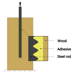
Figure 3: Glued-in rod composite system. [15]
