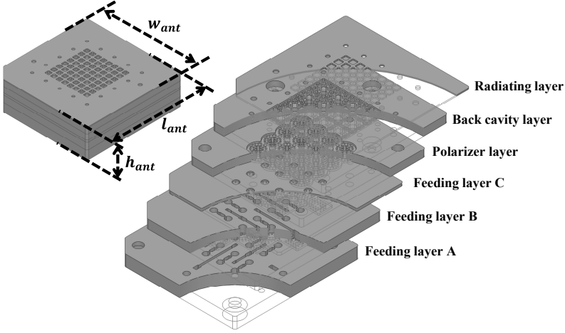
Figure 3.14: Multi-layer structure of the dual-circularly polarized planar array.
