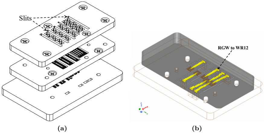
Figure 3.16: a) The proposed multi-layer antenna module. b) Distribution of the antenna elements with vertical transitions to standard WR12 waveguides.
