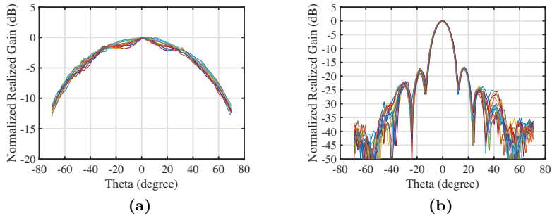
Figure 3.13: Measured radiation patterns of RX slot arrays at 76.5 GHz with all 16 elements plotted together: (a) E-plane, (b) H-plane.
