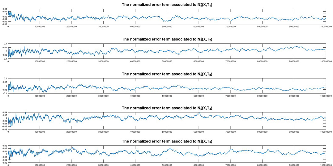
Figure 1. The normalised error terms X^{-\frac{1}{2}}(N_5^+(X, T) - A_5^+(T)X - B_5^+(T)X^{\frac{5}{6}}) for the splitting types T = T_1, \dots, T_5 as described in Section 2.
