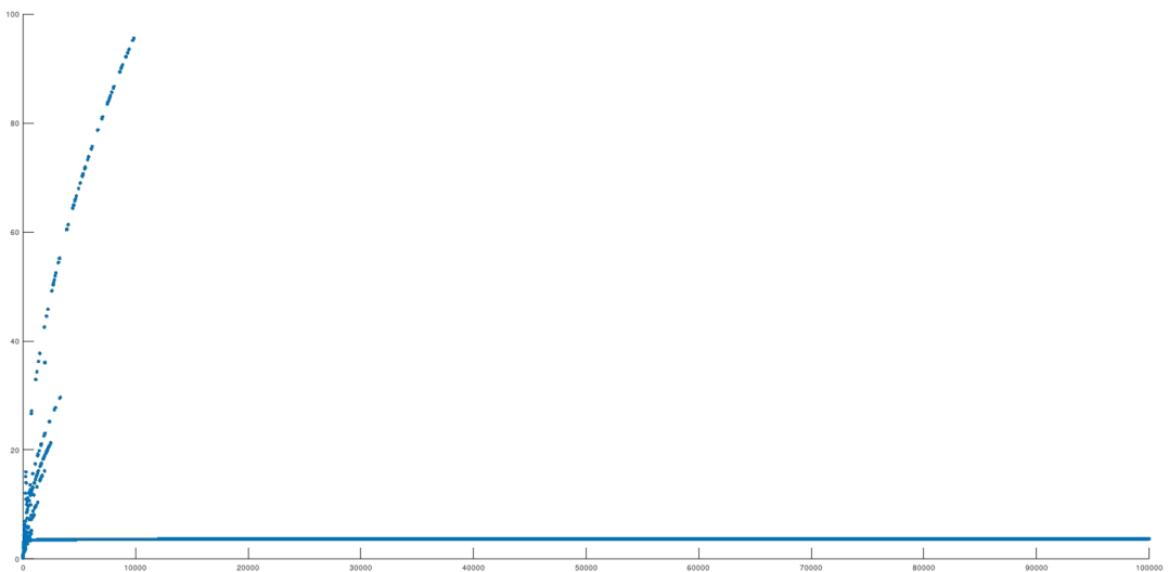
Figure 4. A plot of (p, p f_p(10^4, T_4)) for p < 10^5 .
