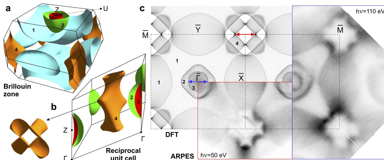
Fig. 5 Fermi surface (FS) for GdRu 2 Si 2 in the paramagnetic phase presented for the first BZ (a) and for the reciprocal lattice unit (b). In panel (b), band 1 is not shown for simplicity; the left outset shows the top perspective view of band 4. (c) Projection of the calculated FS on the (001) surface. The red and blue framed parts show the ARPES-derived FS maps obtained with photon energies of h\nu = 50 eV and h\nu = 110 eV, respectively. The red arrow indicates the proposed nested region in the 3D FS while the blue arrow shows the region near the center of the BZ, which was discussed in ref. 10.
