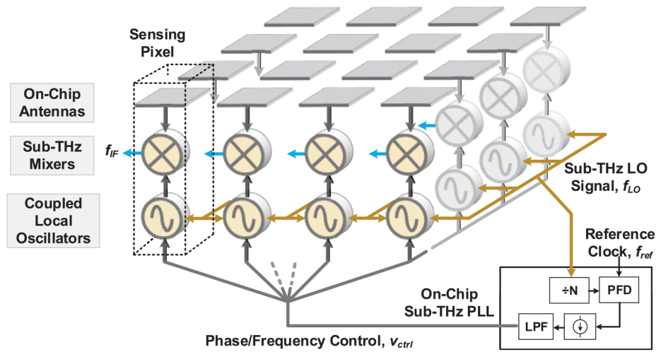
Figure 16. Coupled oscillators technique. LO, Local Oscillator; PLL, Phase-Locked Loops; PFD, Phase Frequency Detector; LPF, Low-Pass Filter. ©2019 IEEE. Reprinted, with permission, from 95.
