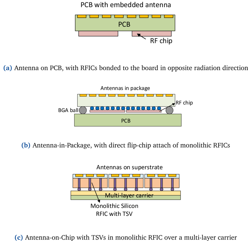
Figure 8. Classification of system packaging implementation diagram with different approaches. RF, Radio Frequency; BGA, Ball-Grid Arrays; PCB, Printed Circuit Board; RFIC, Radio-Frequency Integrated Circuit; TSV, Through Silicon Via.
