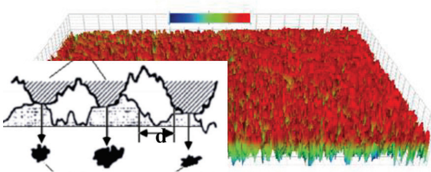
Figure 9 illustration of solid-solid interfacial cavity defects formed by solid material surface roughness (measured abraded surface roughness by P500 sandpaper)
