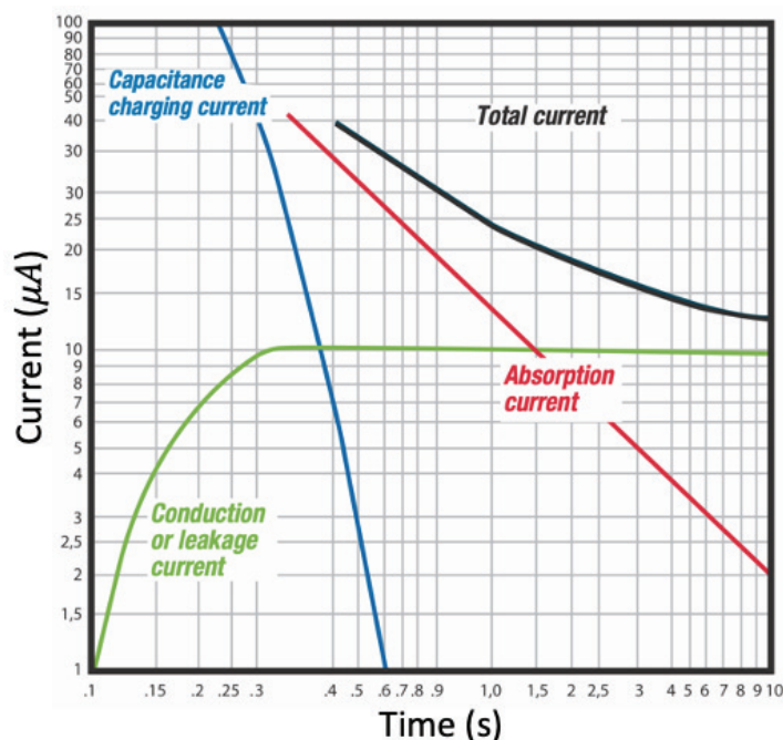
Figure 33. illustration of three main current contributions within the insulation system after being exposed to a DC stress [15].
