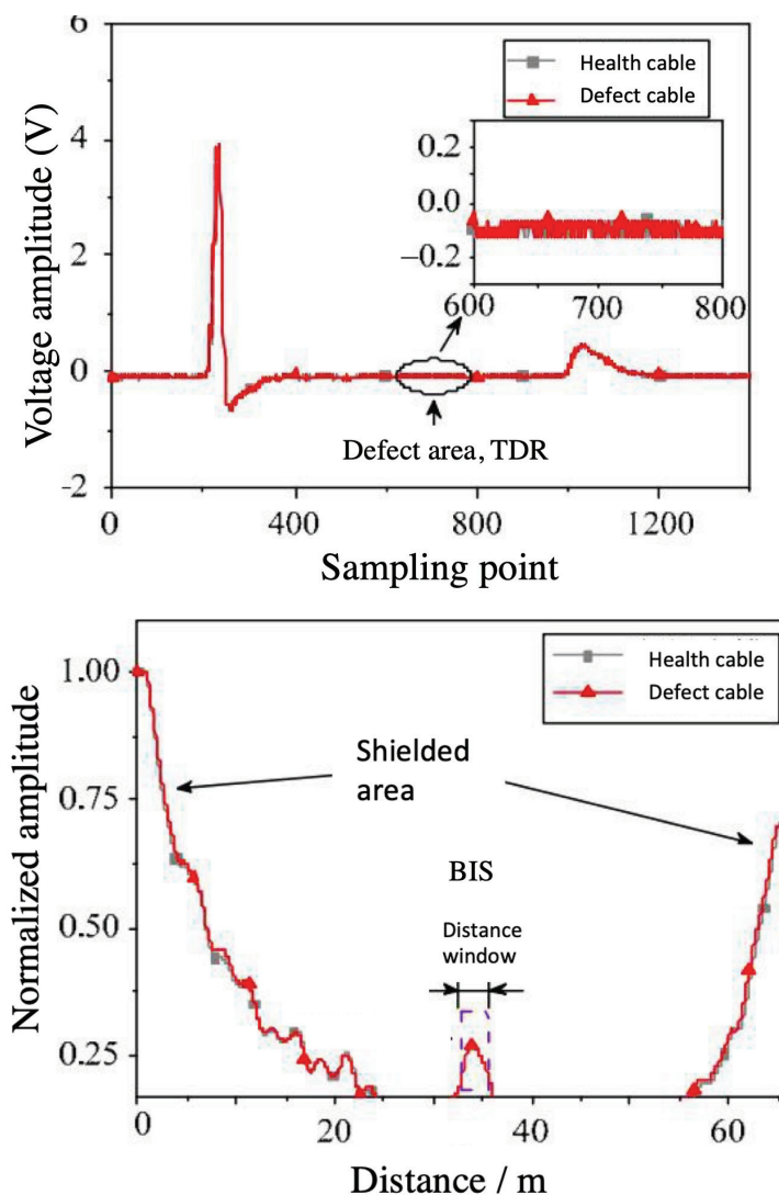
Figure 32 comparison of cable defect detection and localization by using TDR and BIS measurements[13].
