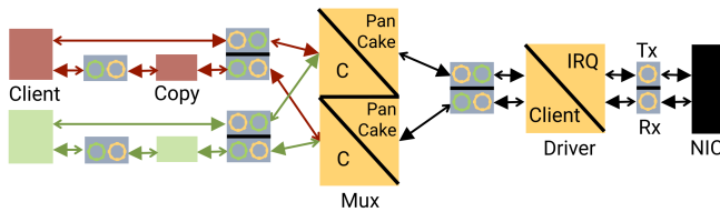
Figure 4. sDDF networking architecture. Coloured boxes are modules, grey boxes shared data structures.
