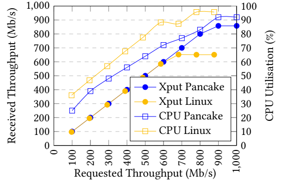
Figure 6. Linux vs Pancake Mux Benchmark
