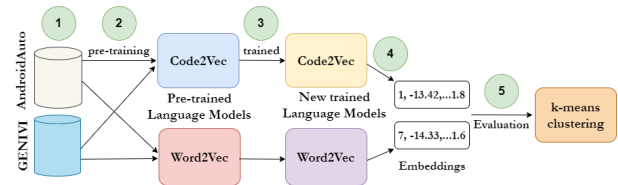
Figure 1: Pre-training with Word2Vec and Code2Vec on Genivi and Android Auto codebases.
