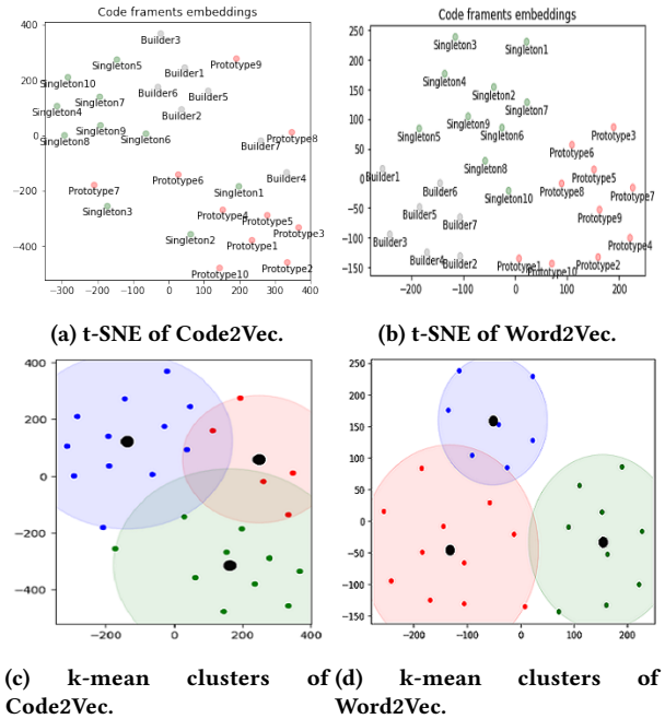
Figure 2: t-SNE and k-mean Clustering Visualizations of different Design Patterns after pre-training PLMs.
