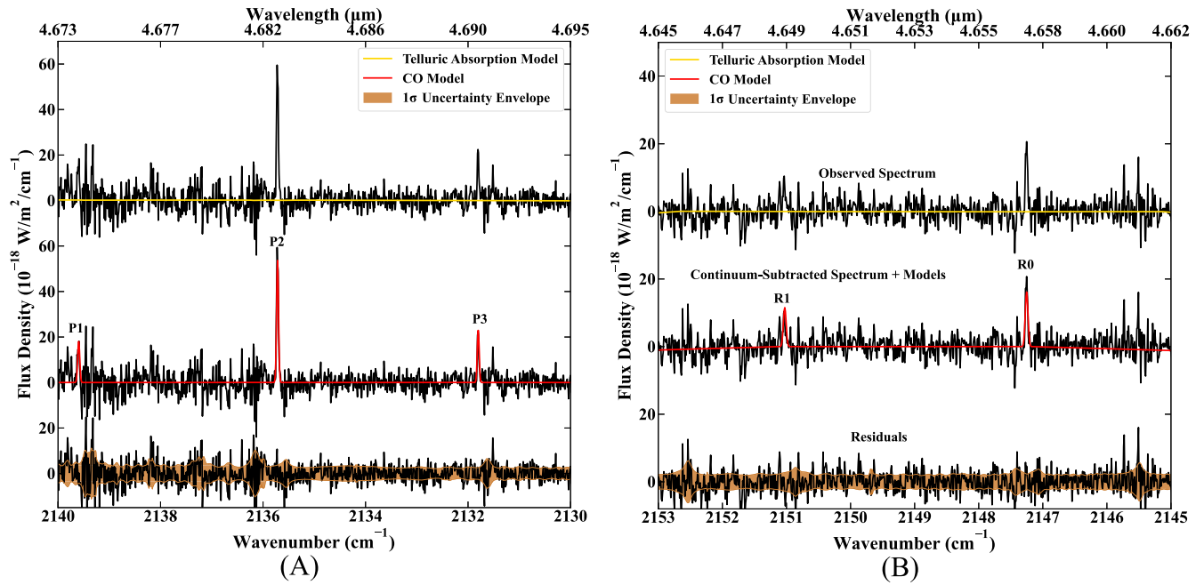
Figure 3. (A)–(B). Extracted IRTF/iSHELL spectra showing detections of CO in SW1 on 2021 October 6 from two separate echelle orders from the M2 setting, (A) order 110 covering 2140–2130 \text{cm}^{-1} and (B) order 111 covering 2153–2145 \text{cm}^{-1} . The uppermost spectrum in each panel is the observed spectrum, with the gold trace showing the telluric absorption model (convolved to the instrumental resolution and scaled to the observed continuum level). Telluric features are only weakly visible, given the weak continuum emission in SW1. The lower spectrum in each panel is the residual emission spectrum (after subtracting the telluric absorption model), with fluorescence models overlain for CO (red) and the 1\sigma uncertainty envelope shaded in bronze. Individual CO rovibrational transitions are labeled.
