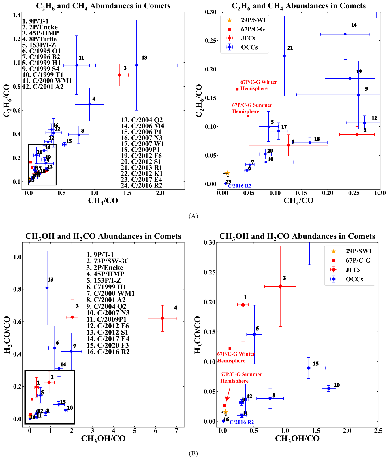
Figure 7. (A) Relative abundances of hypervolatiles in comets (Le Roy et al. 2015; Dello Russo et al. 2016; Biver et al. 2018; McKay et al. 2019). (B) Relative abundances of CH_3OH and H_2CO in comets (Le Roy et al. 2015; Dello Russo et al. 2016; Biver et al. 2018; McKay et al. 2019; Cordiner et al. 2022). Arrows indicate 3\sigma upper limits. Measurements for 67P/Churyumov–Gerasimenko in its summer and winter hemispheres (Le Roy et al. 2015) are indicated. For both figures, the right panel is zoomed in on the region highlighted by the black box in the left panel.
