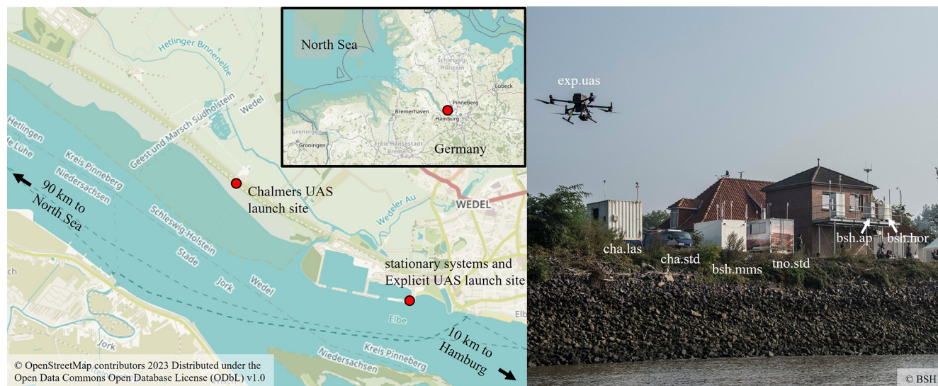
Figure 1. Left panel: location of the measurement site at the northern banks of the Elbe River in Wedel near Hamburg (© OpenStreetMap contributors 2023. Distributed under the Open Data Commons Open Database License (ODbL) v1.0). Right panel: picture of the positioning of the stationary systems as seen from river (© BSH).
