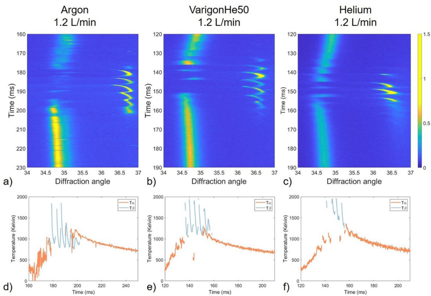
Figure 2. (a–c) Evolution of the diffraction patterns recorded during the scanning of single layers of the 6 \times 6 \text{ mm}^2 samples, displayed as intensity versus diffraction angle and time waterfall plot. The colour scale was capped at 1.5 counts per pixel for visibility. (d–f) Corresponding temperature evolution in the \alpha and \beta phase fields.
