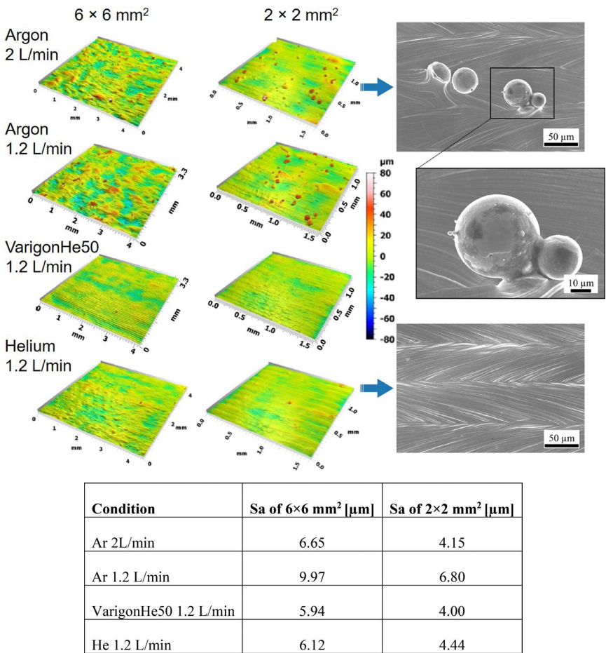
Figure 4. Topography measurements of the produced specimens with the miniature LPBF system using the confocal fusion method for the different process atmosphere conditions.
