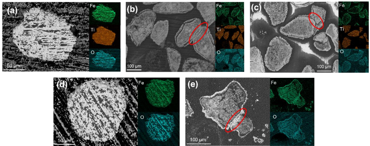
Figure 4.3 The elemental distribution of iron, titanium, and oxygen within (a) fresh ILFC, (b) defluidized ILFC, (c) defluidized ILAU, (d) fresh TOFC, and (e) defluidized TOFC. The red circles indicate interparticle joints.
