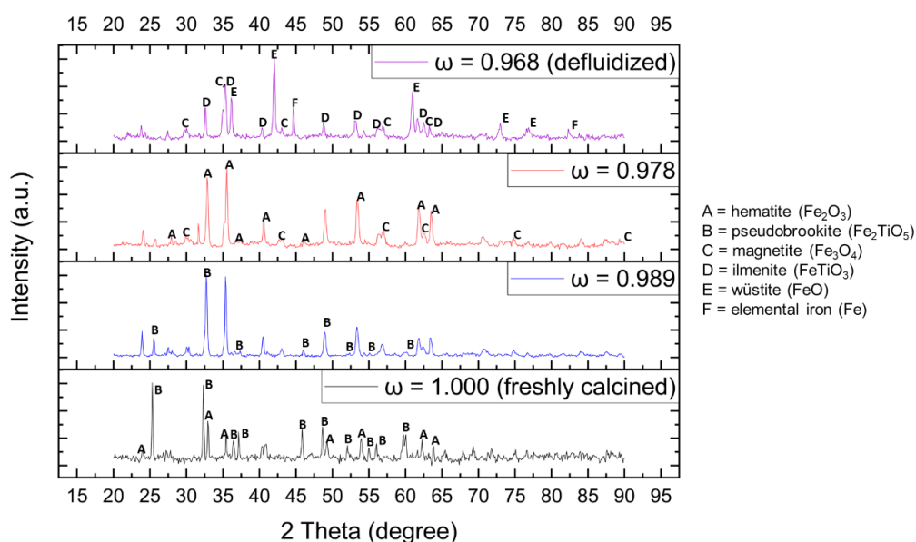
Figure 4.2 Example of diffractograms of the defluidized oxygen carriers, i.e., freshly calcined ilmenite ore (ILFC) in this case, at various mass conversion degrees.
