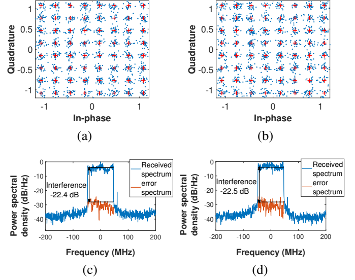
Fig. 19. Constellation and interference of MU-MIMO Case 2 at 93 MHz bandwidth. (a) Constellation of User 1; (b) Constellation of User 2. (c) Interference of User 1; (d) Interference of User 2.
