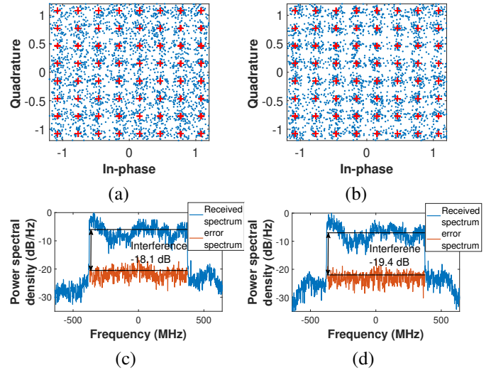
Fig. 20. Constellation and interference of MU-MIMO Case 1 at 748 MHz bandwidth. (a) Constellation of User 1; (b) Constellation of User 2. (c) Interference of User 1; (d) Interference of User 2.
