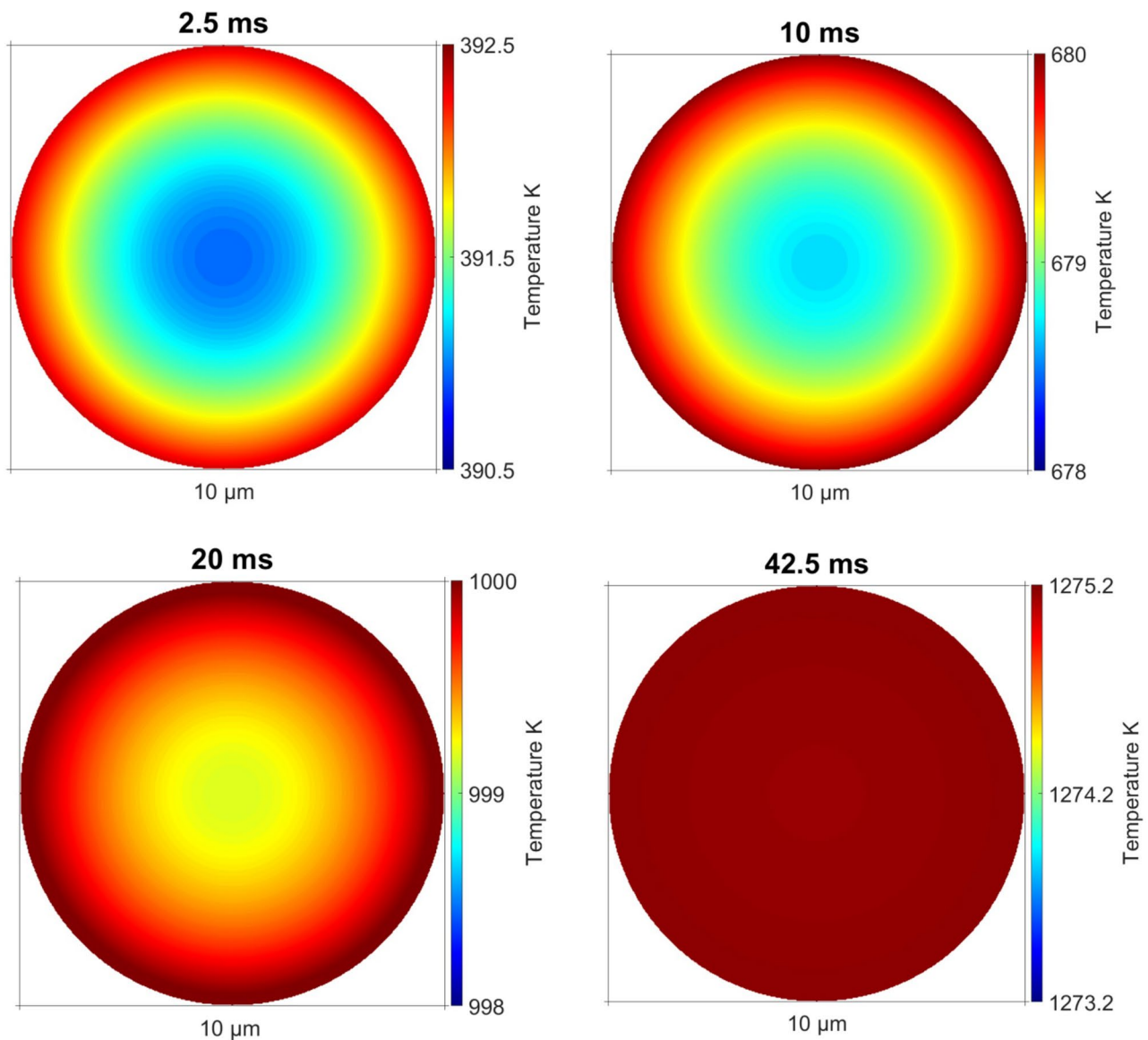
Fig. 7 Modelled cross-section of PF (10 µm diameter and 100 nm susceptor coating) showing edge-to-core temperature distribution at 2.5, 10, 20 and 42.5 ms of MW heating, which correspond to fibre temperatures of approximately 100, 400, 700 and 1000 °C, respectively
