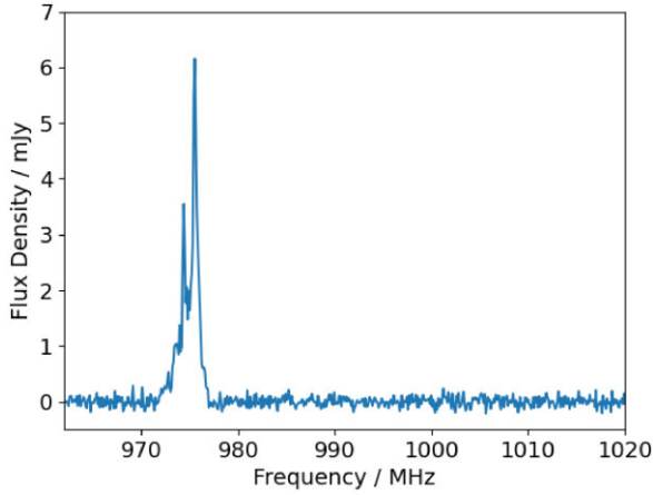
Figure 1. The observed-frame spectrum of the OHM J095903.22+025356.1 from 960 to 1020 MHz. The rms noise across the spectral range spans 70–80 \mu\text{Jy} per 104.5 kHz channel across this range (see Heywood et al., in preparation for further details).
