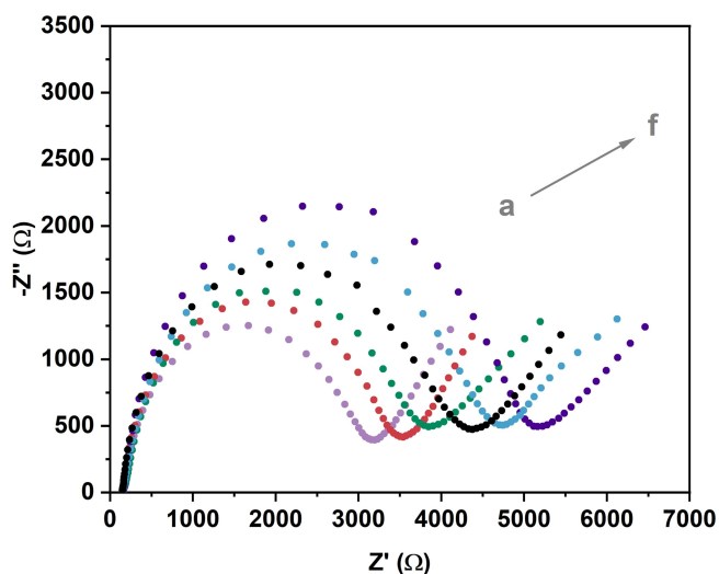
Figure 6. The Nyquist impedance spectra of the anti-IAA/PAMAM/PCN/Au after incubation with different concentrations of IAA (a) 0, (b) 10 ng/mL, (c) 100 ng/mL, (d) 1 µg/mL, (e) 10 µg/mL, (f) 100 µg/mL.
