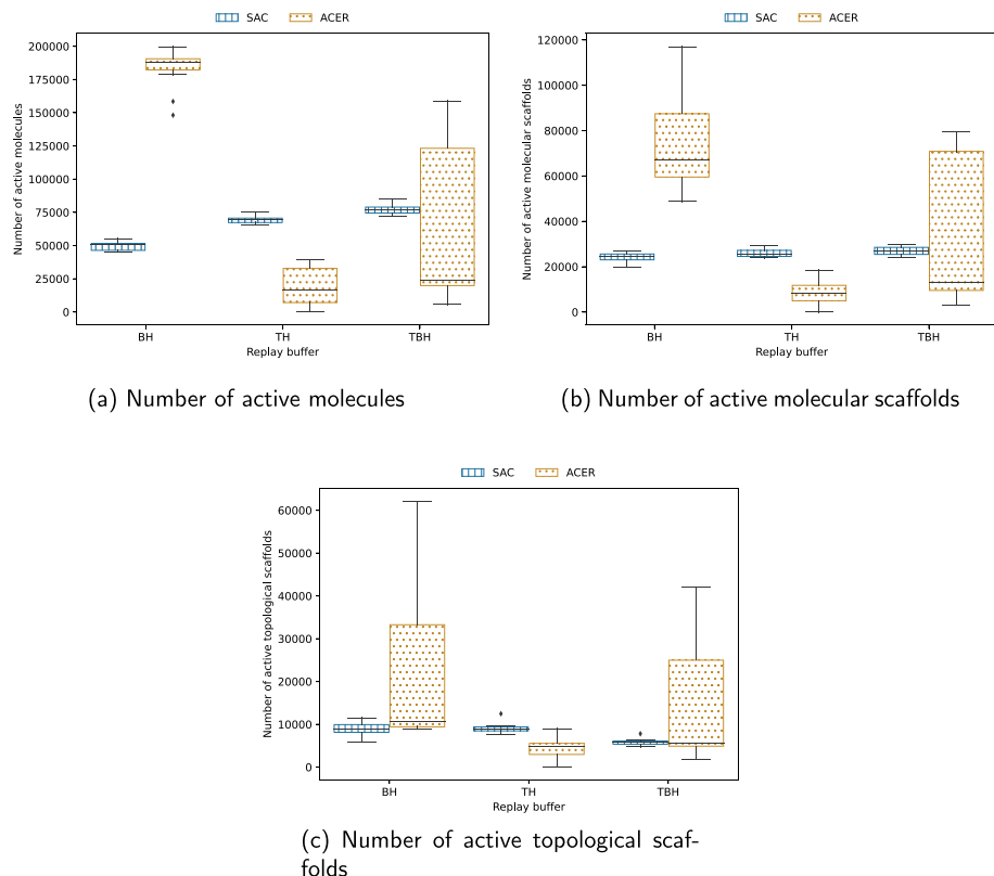
Fig. 9 Box plots of the number of unique active molecules and active scaffolds for the off-policy algorithms ACER and SAC (higher is better) when utilizing identical molecular scaffold filter. The box plot is computed over 11 repeated runs for each combination of policy and replay buffer. 128 SMILES strings are sampled in each episode, with a budget of 2000 episodes in total
