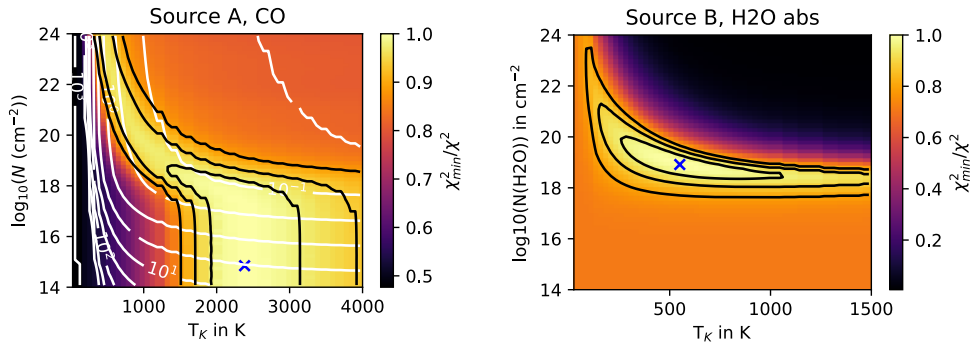
Fig. C.2. As Figure C.1, but for CO emission in source A and H 2 O absorption in source B
