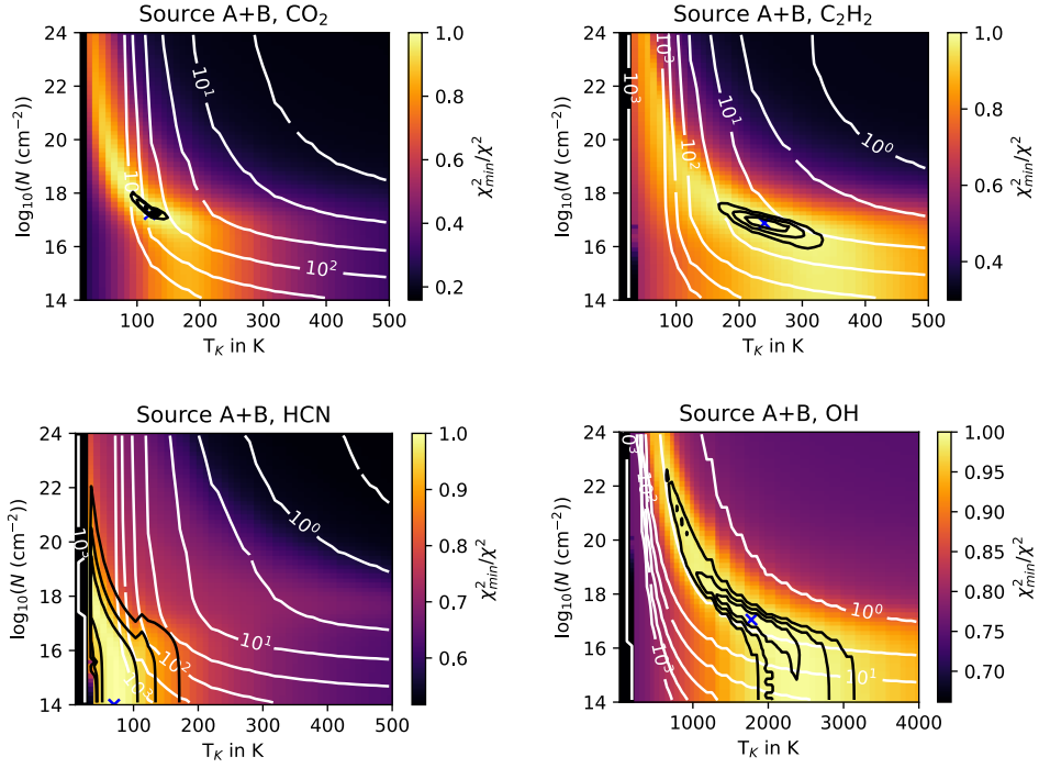
Fig. C.1. Normalized \chi^2 maps (colour scale) of the LTE model temperature and column density grids for CO 2 , C 2 H 2 , HCN, and OH model fits in source A+B. The best-fit emitting radius for each model is overlaid as white contours, while the 1, 2, and 3 \sigma confidence interval contours are overlaid in black. The best-fit model at the minimum \chi^2 is shown by a blue cross.
