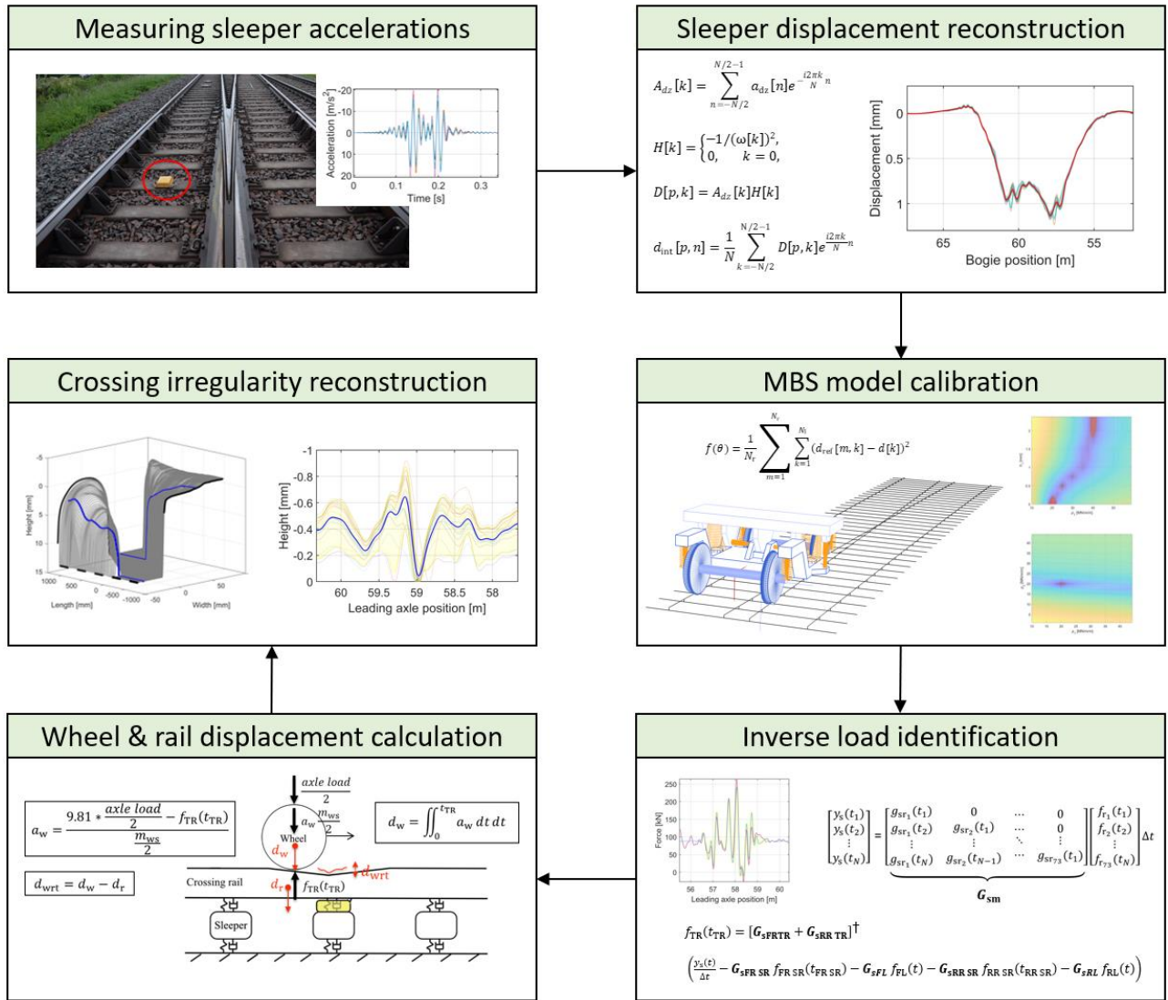
Figure 12 Crossing Panel Condition Monitoring system framework
