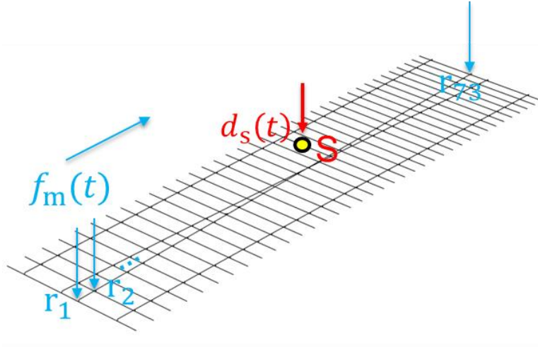
Figure 26 Single Green's function spatial input-output relation and used track structure model.
