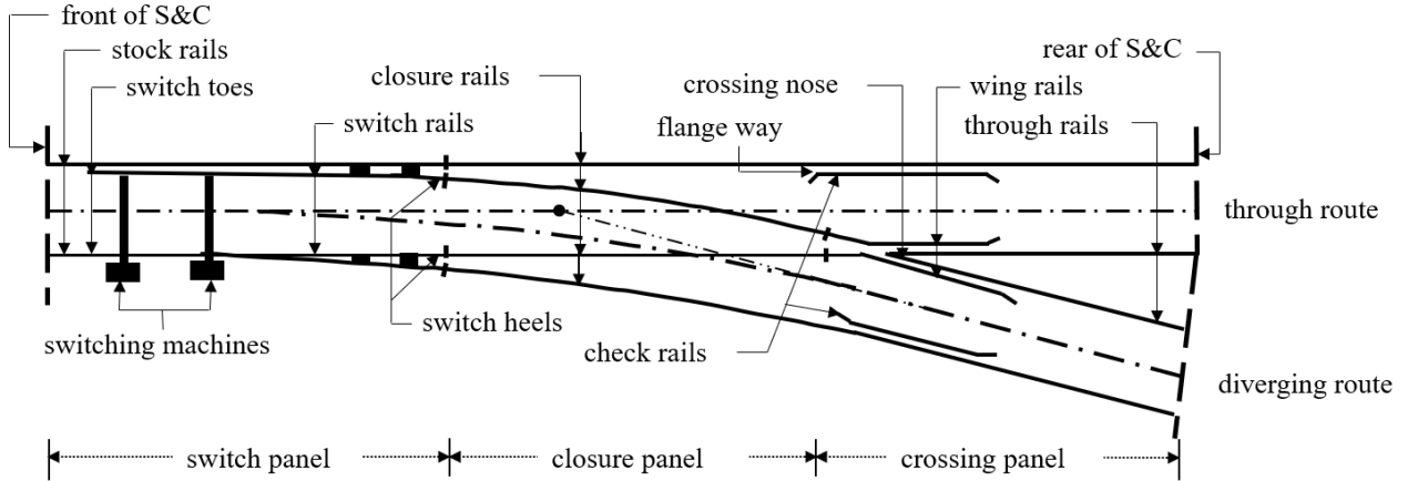
Figure 2. Layout, components, and nomenclature for a standard right-hand side S&C with a fixed crossing [9].
