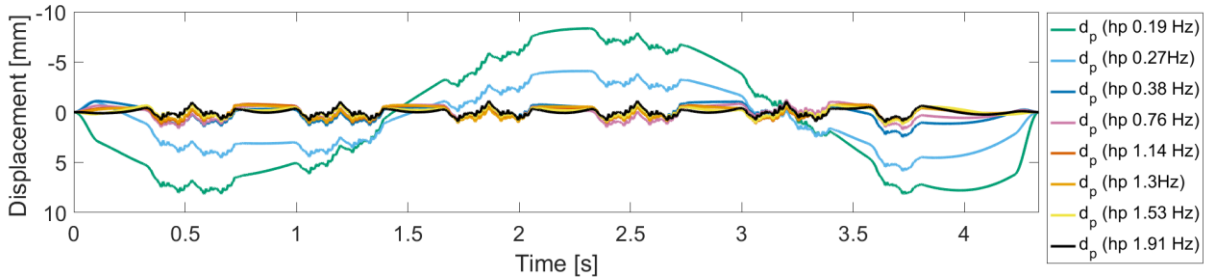
Figure 23 Integrated sleeper displacement for different high-pass frequencies f_p before in-between-bogie baseline detrending.
