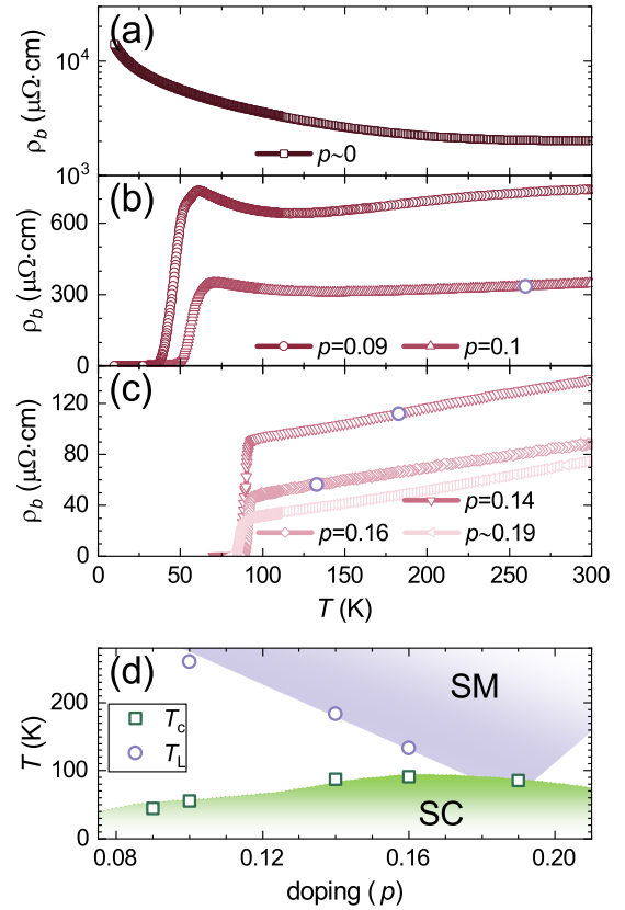
FIG. 7. Doping dependence of nanoribbon resistivity. Panels (a)–(c) show \rho_b(T) for various 300 nm thick films at different oxygen doping levels. The critical temperature T_c for each film is determined from the maximum of the first derivative of \rho_b(T) . T_L (violet circles), marking the crossover between the pseudogap region and the strange metal phase, is the temperature below which the resistivity \rho_b(T) deviates by 1% from the high-temperature linear fit of the curves, performed in the interval 280 \text{ K} < T < 300 \text{ K} . Notably, all \rho_b(T) datasets are extensive, featuring a sub-Kelvin temperature step size. Panel (d) presents a phase diagram constructed from the obtained values of T_c and T_L , exhibiting good agreement with the superconducting (SC) and strange metal (SM) regions observed in YBCO single crystals and c -axis oriented films [52,68].
