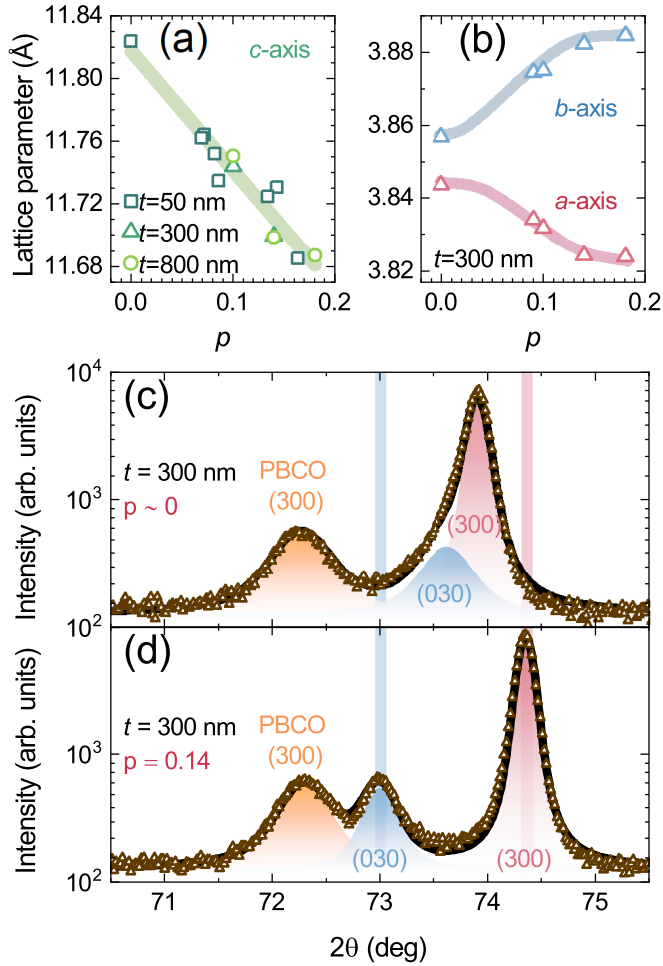
FIG. 4. Locking of the \text{CuO}_2 planes in a -axis oriented YBCO films. (a) The c -axis parameter, extracted from the (\ell 0 0) and (\ell 0 n) Bragg reflections, is shown as a function of the doping p for films of different thickness. For each sample, p has been determined based on the c -axis length, and then utilizing the critical temperature T_c measured via transport (see Sec. IV) and the empirical parabolic relationship connecting doping and T_c in cuprate HTS [52,61]. Notably, all data points for the 50 nm thickness have been collected from a single, multiply annealed thin film. (b) The a - and b -axis parameters, extracted from the (\ell 0 0) and (\ell m 0) Bragg reflections, are plotted vs p for different 300 nm thick films. (c), (d) The symmetrical 2\theta - \omega scans respectively of an insulating ( p \sim 0 ) and of an underdoped ( p = 0.14 ) film are compared. The decomposition of the data into three Voigt profiles associated to the (300) PBCO, the (030) YBCO, and the (300) YBCO reflections shows first that the PBCO layer is unaffected by the annealing procedure, as the peak position is unchanged vs doping, and second, that the two YBCO peaks, related to the \text{CuO}_2 planes, are distinct, even though they get closer, in the undoped sample. To facilitate the comparison, the vertical bars show the position of the two YBCO peaks in the doped sample.
