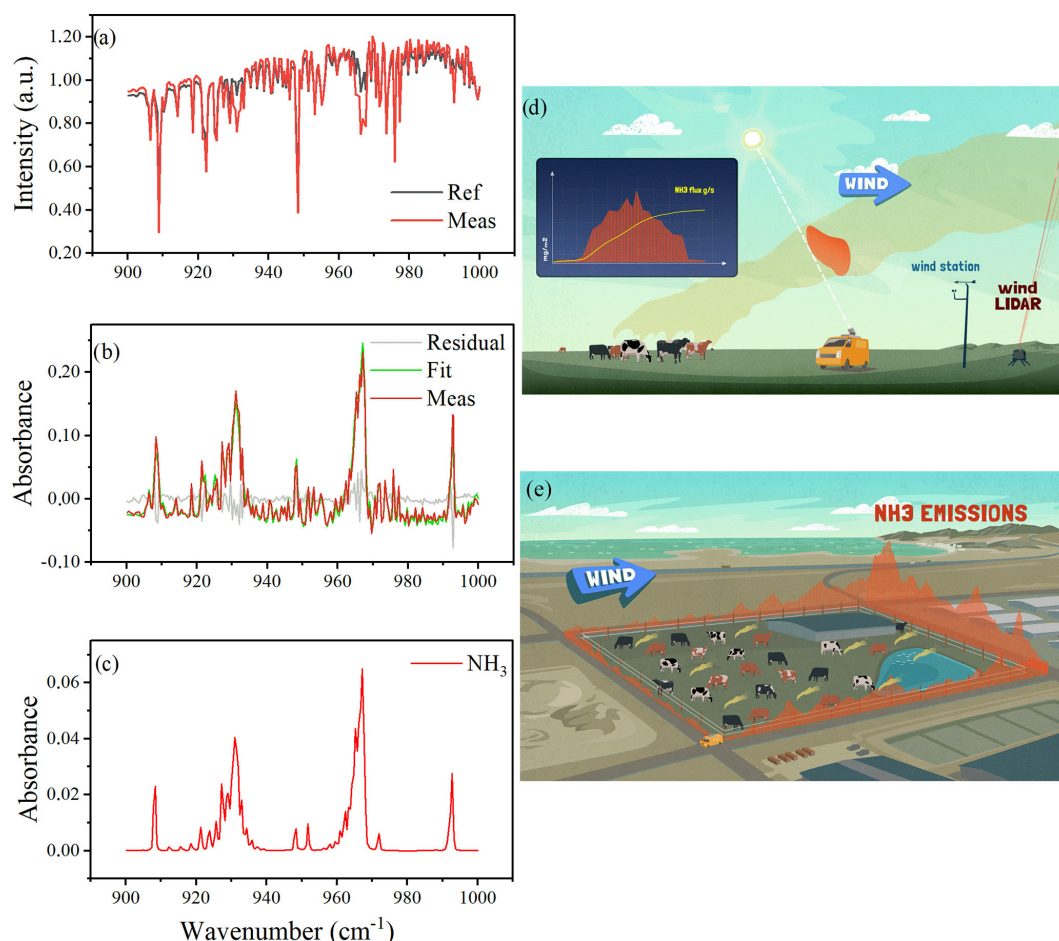
Figure 1. (a) Example of spectra measured in the plume and in the background. (b) Measured and fitted absorbance spectra and the calculated residual spectra. (c) NH 3 calibration absorbance used to model the fitted spectra (approx. 40 mg m -3 ). (d) Example of solar spectral measurements when crossing the target plume. (e) Example of a box measurement around a target farm.
