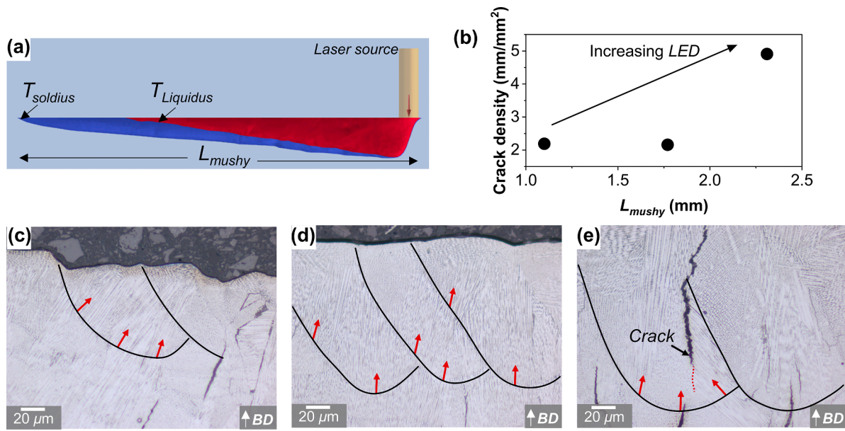
Fig. 10. (a) Simulation showing the melt pool + mushy zone for LED of 0.3 J/mm showing the length of the mushy zone ( L_{mushy} ) along with the solidus and liquidus temperatures used for the isosurfaces. (b) Correlation between the length of the mushy zone from the simulation and crack densities for different LEDs shown in (c)-(e). The simulation was done using the Additive Manufacturing Module in ThermoCalc 2024a. TCNI12 database was used for calculating the Scheil solidification curve. (c)-(e) LOM etched micrographs showing melt pools for samples processed with LED of (c) 0.1 J/mm, (d) 0.2 J/mm and (e) 0.3 J/mm.
