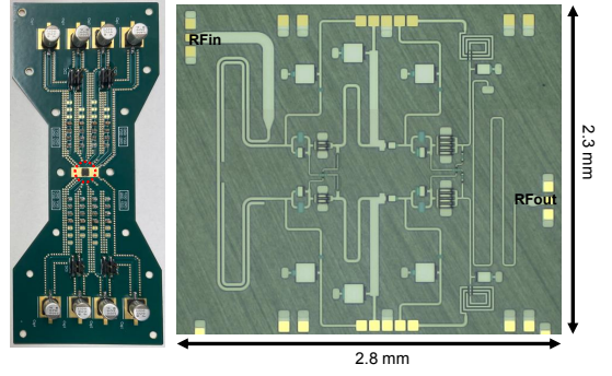
Fig. 5. (a) The test PCB board and (b) chip photograph of the fabricated prototype (Total chip area: 2.8 \text{ mm} \times 2.3 \text{ mm} including DC and RF pads).
