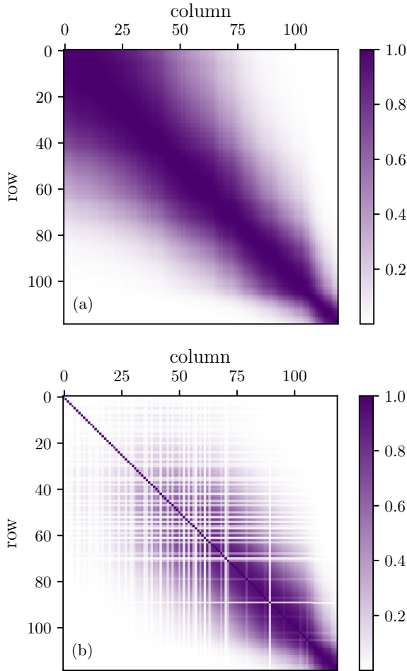
FIG. 5. Correlation matrices based on the NNLO covariance matrix \Sigma_{\sigma_{\text{tot}}} of the 119 \sigma_{\text{tot}} data. In panels (a) and (b) we exclude and include, respectively, the experimental variances \Sigma_{\text{exp},\sigma_{\text{tot}}} . The data are sorted by energy in increasing order.
