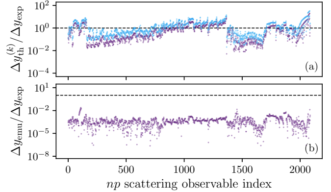
FIG. 6. The EFT truncation and EC emulator errors compared to experimental errors for all considered np scattering data. (a) The standard deviations of the EFT truncation errors at NLO and NNLO. (b) The NNLO EC emulator errors ( \Delta y_{\text{emu}} ). Colors as in Fig. 2. In both panels we divide by the the experimental 1\sigma errors ( \Delta y_{\text{exp}} ) and the horizontal dashed lines indicate a ratio of 1.
