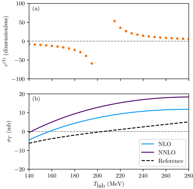
FIG. 2. (a) Calculated expansion coefficients for \sigma_T . (b) The NLO, NNLO, and reference values from which the coefficients are calculated. Note the zero crossing for the reference value at T_{\text{lab}} \approx 205 MeV.
