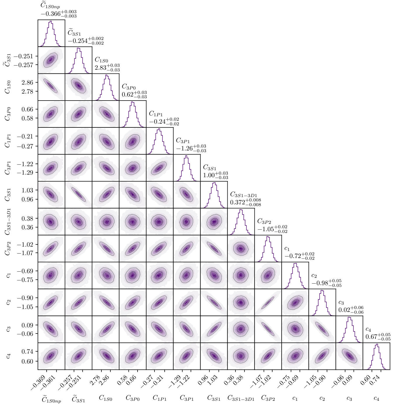
FIG. 12. Posterior PDF of the values for the LECs at NNLO inferred using a correlated model for the EFT truncation error. See Fig. 9 for figure notation.
