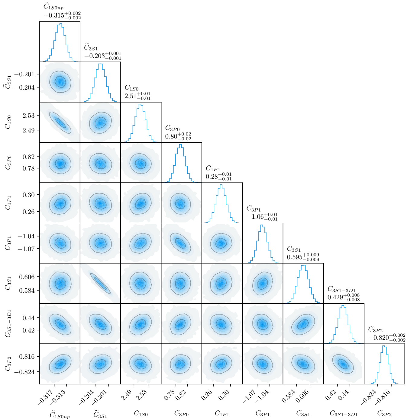
FIG. 9. Posterior PDF of the values for the LECs at NLO inferred using an EFT truncation error in the uncorrelated limit. The inner (outer) gray contour line encloses 39% (86%) of the probability mass. The dot-dashed vertical lines indicate a 68% credibility interval in the univariate marginals. See main text for units and conventions.
