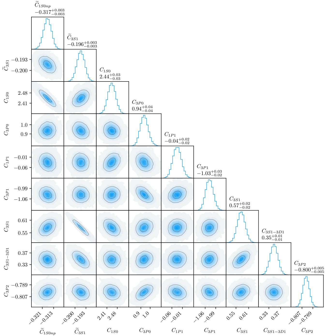
FIG. 10. Posterior PDF of the values for the LECs at NLO inferred using a correlated model for the EFT truncation error. See Fig. 9 for figure notation.
