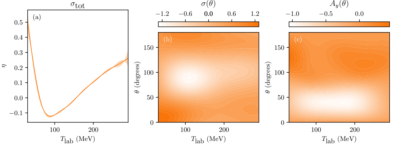
FIG. 4. Mean \mathcal{GP} predictions \eta for (dimensionless) expansion coefficients for (a) \sigma_{\text{tot}} , (b) \sigma(\theta) , and (c) A_y(\theta) . The light colored band in (a) indicates a 95% credible interval.
