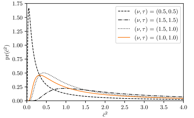
FIG. 3. The inverse- \chi^2 prior \text{pr}(\bar{c}^2|I) (orange) for the \mathcal{GP} hyperparameter \bar{c}^2 . Shown in black are alternative priors that we use to show the robustness of the inference.
