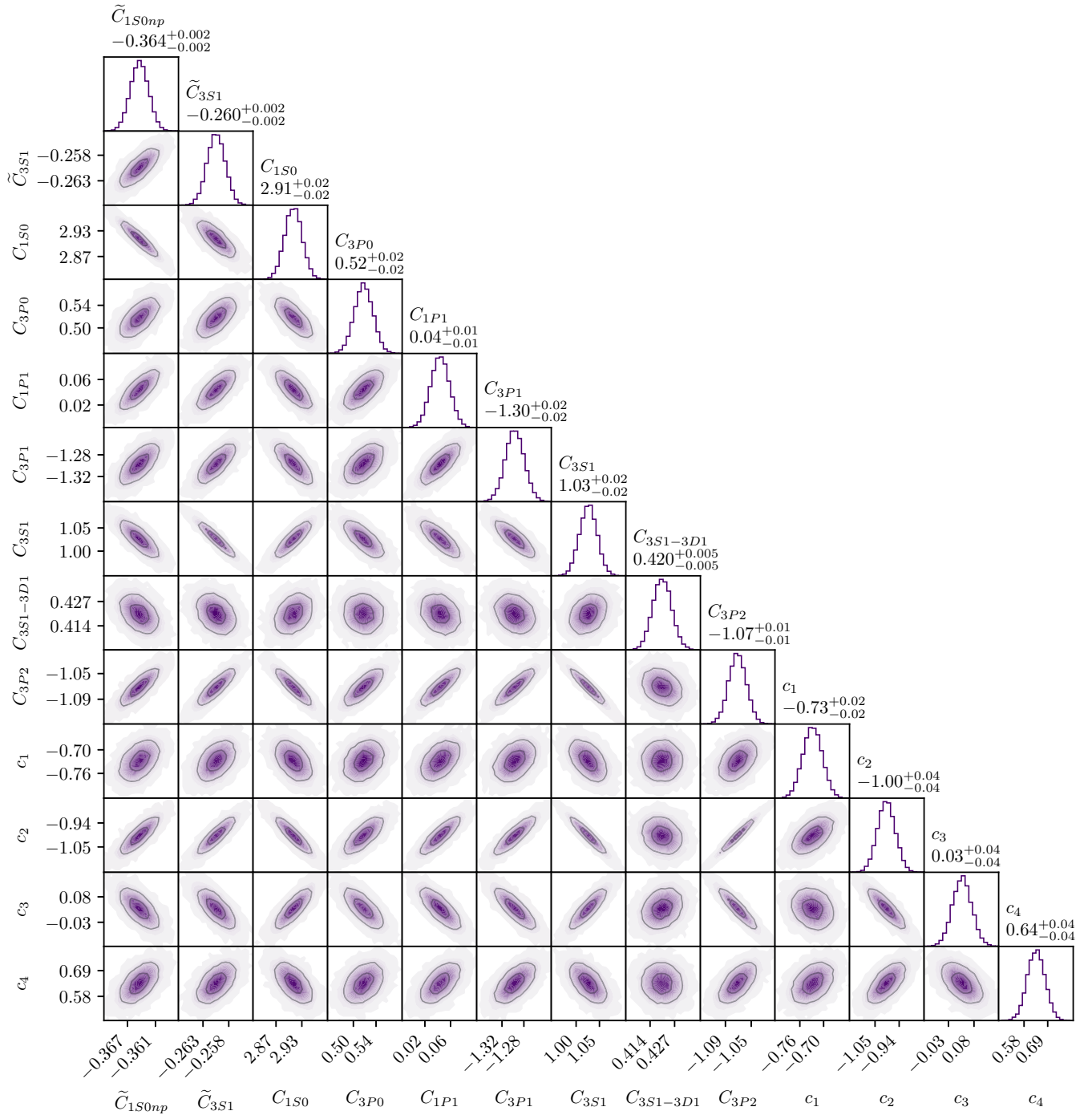
FIG. 11. Posterior PDF of the values for the LECs at NNLO inferred using an EFT truncation error in the uncorrelated limit. See Fig. 9 for figure notation.
