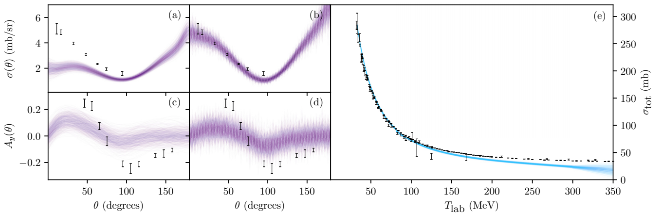
FIG. 8. 500 draws from the PPDs for unseen data for (a) \sigma(\theta) at NNLO and T_{\text{lab}} = 319 MeV with a correlated error, and experimental data from Ref. [67]. (b) Same as (a) but with an uncorrelated error. (c) A_y(\theta) at NNLO and T_{\text{lab}} = 350 MeV with a correlated error, and experimental data from Ref. [68]. (d) Same as (c) but with a correlated error. (e) \sigma_{\text{tot}} at NLO and T_{\text{lab}} = 30\text{--}350 MeV (see Ref. [42] for references to the experimental data).
