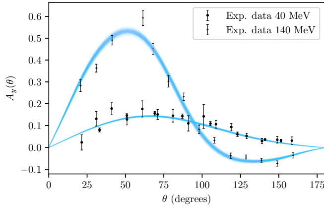
FIG. 7. 500 draws from the NLO PPDs for A_y(\theta) at T_{\text{lab}} = 40 MeV and T_{\text{lab}} = 140 MeV using a correlated truncation error. The experimental data at 40 and 140 MeV are from Refs. [64,65] and [66], respectively.
