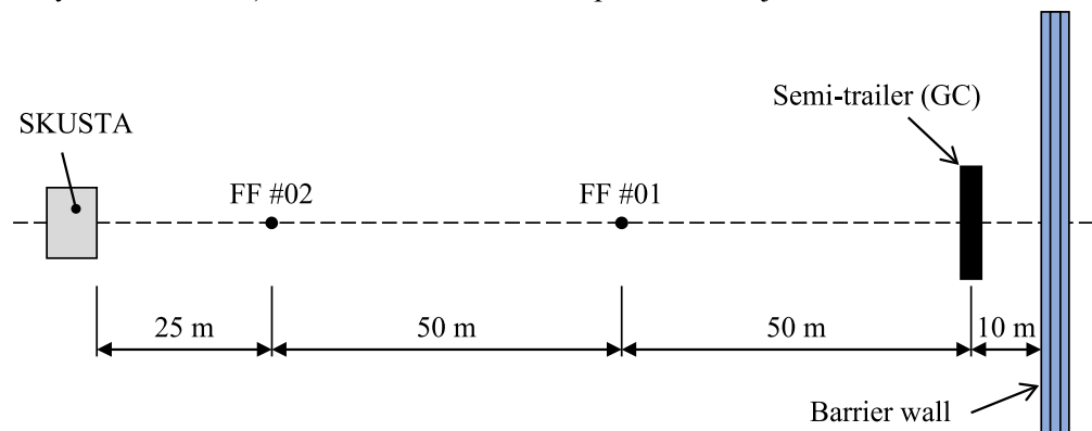
Figure 1. Schematic overview of test-site (plan view), charge placed in semi-trailer at ground zero (GC)
