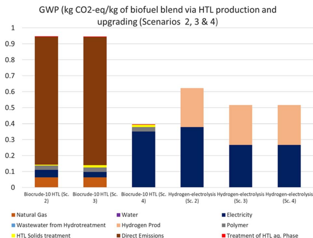
Fig. 9 LCA of HTL biocrude production and upgrading for Scenarios 2, 3 and 4. Scenario 2: total value of GWP metric 0.75 kg CO 2 -eq. per kg biocrude (or 0.02 kg CO 2 -eq. per MJ biocrude) and 1.57 kg CO 2 -eq. per kg (or 0.04 kg CO 2 -eq. per MJ) of fuel blend (diesel, naphtha). Scenario 3: total value of GWP metric 0.74 kg CO 2 -eq. per kg biocrude (or 0.02 kg CO 2 -eq. per MJ biocrude) and 1.46 kg CO 2 per kg (or 0.03 kg CO 2 -eq. per MJ) of fuel blend (diesel, naphtha). Scenario 4: total value of GWP metric 0.31 kg CO 2 -eq. per kg biocrude (or 0.01 kg CO 2 -eq. per MJ biocrude) and 0.91 kg CO 2 per kg (or 0.02 kg CO 2 -eq. per MJ) of fuel blend (diesel, naphtha). Impacts of hydrotreatment/hydrocracking are not shown as they are negligible.
