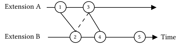
Figure 3: Example of two extensions with reviews and the connections ATW makes. The dotted line shows non-maximizing connections that discrete optimization will remove.
