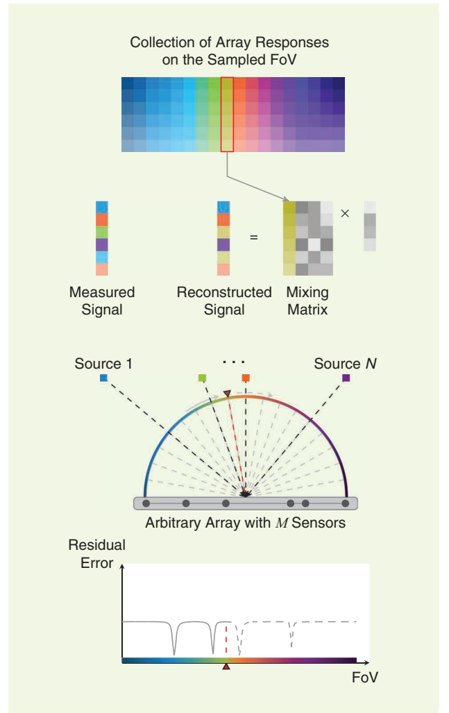
FIGURE 3. An illustration of the PR concept. The optimization is carried out over the relaxed array manifold \mathcal{A}_N , where the structure of the first column in \mathbf{a}(\theta_1) is maintained and the structure of the remaining columns is relaxed to an arbitrary complex matrix, [\mathbf{a}(\theta_2), \dots, \mathbf{a}(\theta_N)] \rightarrow \mathbf{B} \in \mathbb{C}^{M \times (N-1)} . Unlike the single-source approximation, the influence of the remaining source signals during the spectral search is considered by the unstructured matrix \mathbf{B} (depicted by gray columns in the mixing matrix), which generally leads to an improvement of the DoA estimation when sources are closely spaced.
