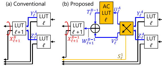
Fig. 5: Inter-layer connection in HiDM decoding.
