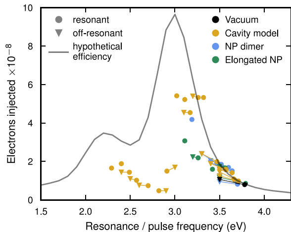
Figure 3. Number of electrons injected into the molecule for different setups. Because the principal charge-transfer excitation is red-detuned relative to the LSP resonance, transferring the most charge requires a trade-off between being tuned to the resonance (circles) and being tuned to the charge-transfer excitation. Imagining that we could “artificially” shift the resonance yields the solid gray line. The slight blue-shift of the in-cavity envelope and the artificially shifted resonance can be attributed to self-polarization effects. 47,52 The data is normalized to correspond to the same absorption as the 201-atom vacuum system. In particular, the values for the NP dimer have been halved, and the values for the elongated NPs have been multiplied by 201 and divided by the number of atoms in each structure.
