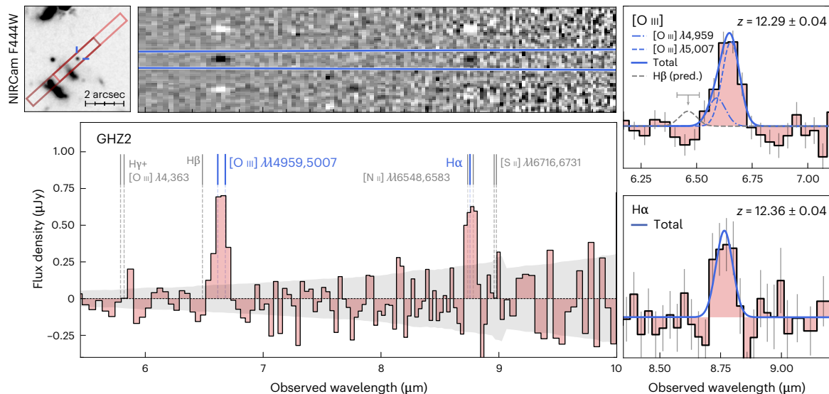
Fig. 1 | JWST/MIRI spectrum of GHZ2 at z = 12.33 . Top left: NIRCcam F444W cut-out image ( 5'' \times 5'' ) centred at the position of GHZ2, with the MIRI/LRS slit illustrated with the red rectangle (at the two different dither positions). The combined 2D spectrum and the aperture used for the 1D extraction are also plotted (see details in Methods). Bottom left: 1D extracted spectrum at the position of GHZ2 across the most sensitive wavelength range, \lambda_{\text{obs}} \approx 5.7\text{--}10 and the associated 1\sigma uncertainty (grey region). The expected wavelengths of typically bright rest-frame optical emission lines are indicated with the vertical
