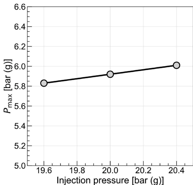
Fig. 10. Maximum explosion overpressures measured for black mass C at the dust concentration of 300 \text{ g/m}^3 and an ignition energy of 20 kJ.
