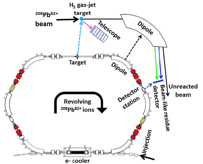
FIG. 1. The lower part shows a schematic view of the ESR. The upper part shows the portion of the ring where our detectors were installed. The trajectory of the scattered protons is represented by the pink arrow and the one of the beam is represented by the black arrow. The trajectories of the heavy beamlike residues produced after emission of \gamma rays ( ^{208}\text{Pb}^{82+} ) and a neutron ( ^{207}\text{Pb}^{82+} ) are indicated by the blue and green arrows, respectively.
