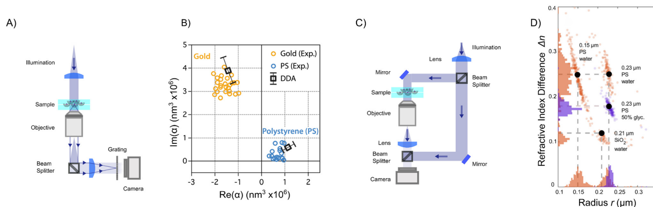
Fig. 14 Particle characterization using holographic imaging. (A) and (B) Using quadrilobe lateral shearing interferometry (QLSI), in ref. 67 it was demonstrated that gold and dielectric nanoparticles can be distinguished based on their complex-valued polarizabilities. (C) and (D) In ref. 19 it was demonstrated that deep learning enhanced analysis of particle scattering patterns recorded in off-axis holography is capable of quantifying the size and refractive index of suspended subwavelength particles. Figure reprinted with permission under the CC-BY 4.0 license.
