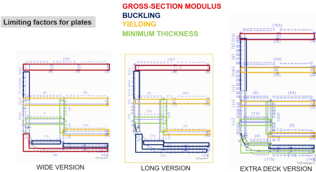
Figure 12 The limiting factors the govern the weight optimization of the three design variants.
