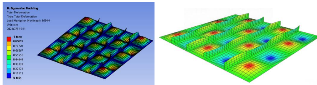
Figure 3-3: First local buckling eigenmode from linearized FEA (left) and PULS (right) under the in-plane loads from the longitudinal X-direction.
