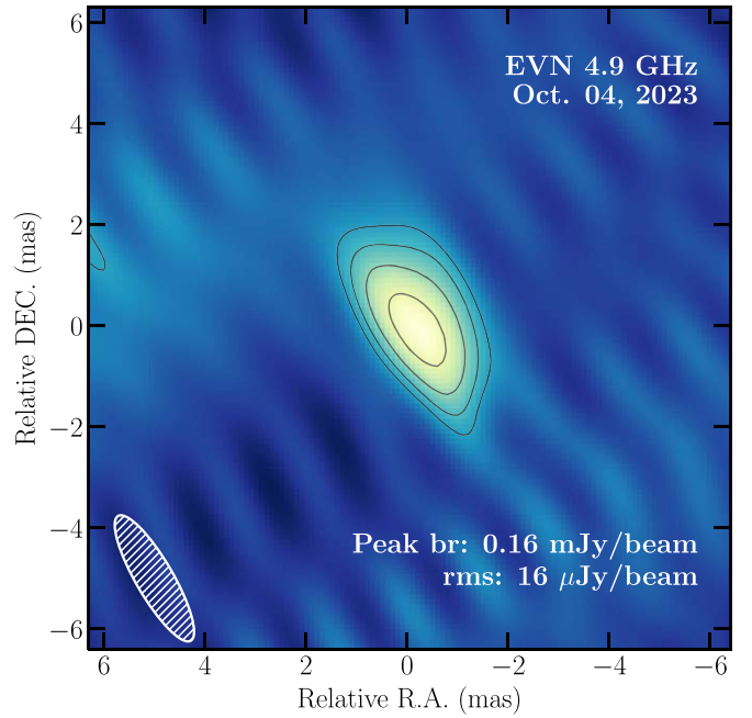
Figure 1. Naturally weighted image of AT2019wey obtained with the 4.9 GHz EVN observation on 2023 October 4. The peak brightness value and the image noise level are labeled in the lower-right corner. Contours start from 3\sigma noise level and increase by a factor of \sqrt{2} . The FWHM of the Gaussian synthesized beam is represented by an ellipse in the lower-left corner ( 2.86 \times 0.73 mas 2 , major axis position angle PA = 30^\circ 2 ).
