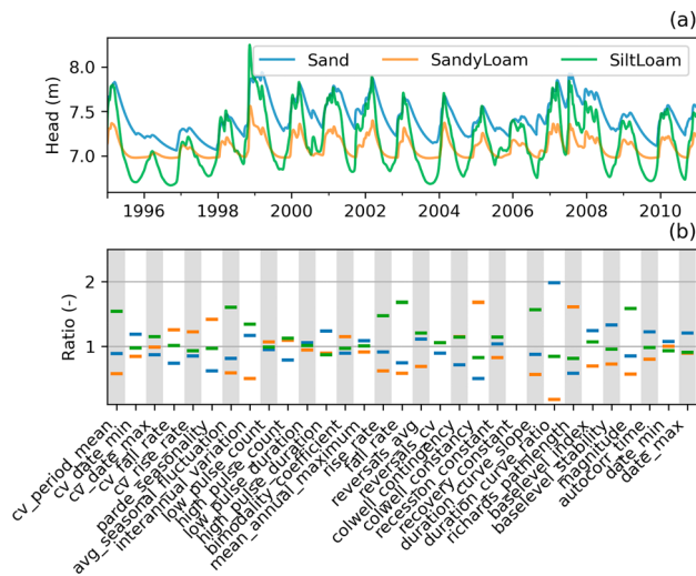
Figure 2. Three selected time series of hydraulic heads (a) and the related normalized groundwater signatures (b). To test the discriminatory power of the signatures, the signatures were normalized by dividing by the mean of each signature for the three heads. The virtual boreholes of the selected time series are located at 1/4 of the distance between the parallel rivers (see Vonk et al. 2024, for more details).
