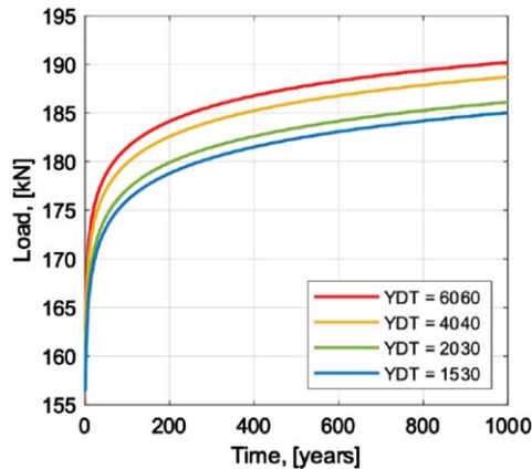
Fig. 8. Extrapolation of loads for a return period of 1000 years.
