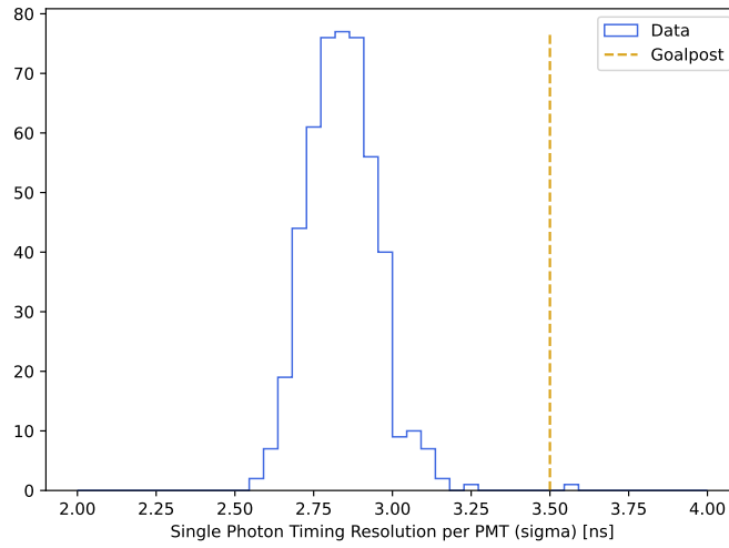
Figure 5: Per PMT single photon timing resolution (SPTR) determined at -40^\circ\text{C} ambient temperature. The yellow line indicates the upper-bound for acceptable timing resolutions to sufficiently resolve characteristic interactions in IceCube at distances around 30 m [8].
