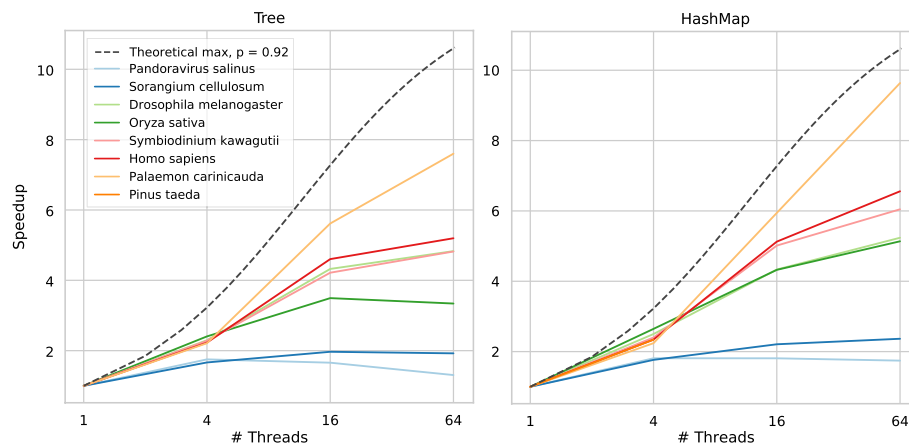
Fig. 8 The parallel speedup of the Tree and HashMap algorithms. The speedup is compared with the theoretically optimal speedup for p = 0.92 given by Amdahl's law. By profiling, we measured that approximately 8% of the code is serial and cannot be accelerated, although this number differs somewhat depending on sequence size and parameters. For short sequences the speedup is small, but longer sequences have close to optimal speedup. The benchmarking machine has 32 cores, and thus the result for 64 threads illustrates that there are some benefits to scheduling more threads than cores. The HashMap exhibits better parallelisation speedup overall
