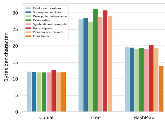
Fig. 7 Memory per input character for the construction of each algorithm. Results for the Pinus taeda are missing for Tree due to insufficient memory on the benchmark server. Overall, Cunial is superior to the other approaches
