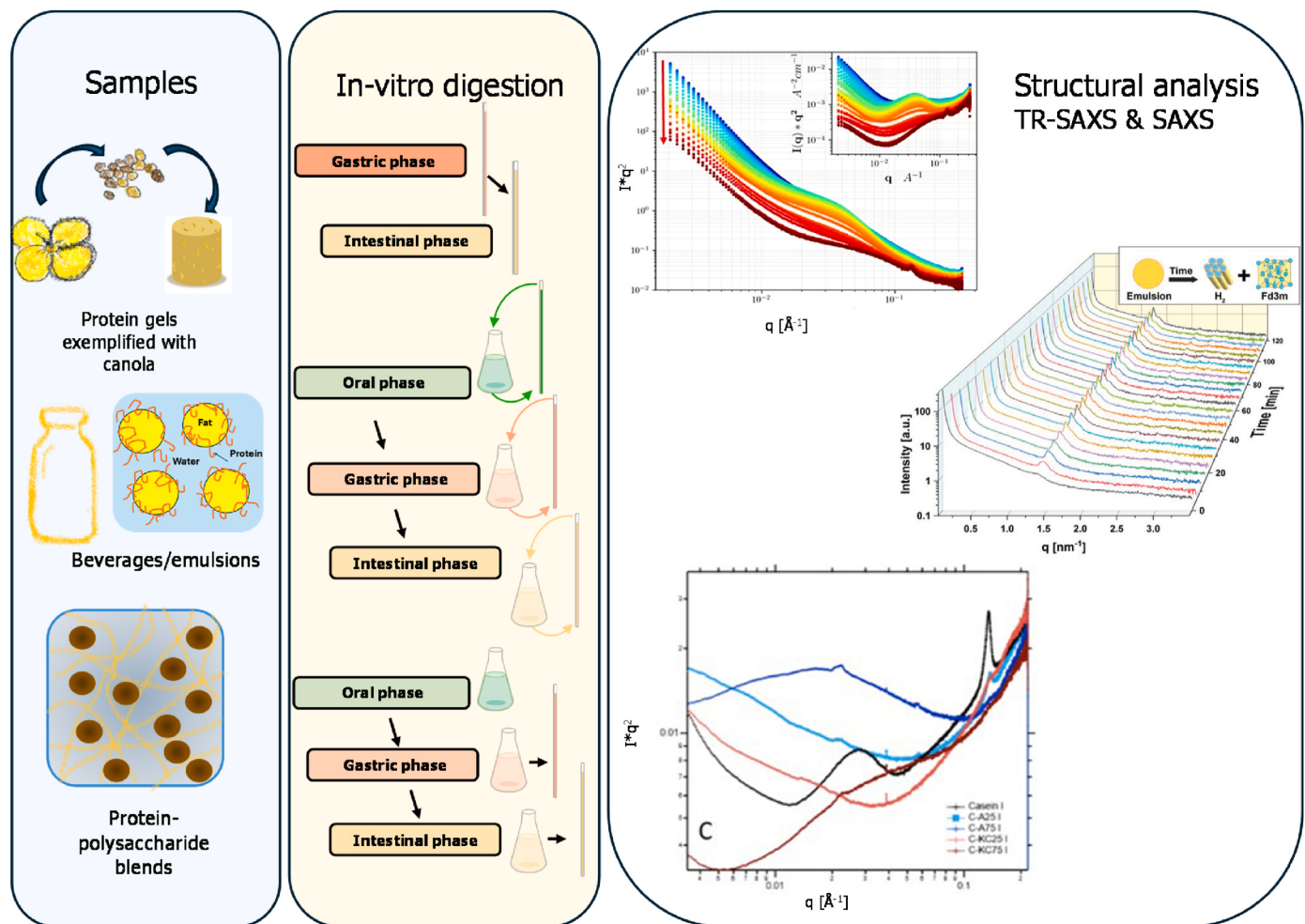
Fig. 5. Structure formation and break-up of protein gels, lipids in beverages, proteins within polysaccharide gels or in presence of polysaccharides (left) during the different phases of digestion (middle) have been monitored using SAXS and time resolved (TR) - SAXS (right). Top image right depicts the scattering profile of canola proteins during digestion (Napieraj et al., 2024), middle right depicts structure formation of buriti oil emulsion during digestion (Freire et al., 2023), and lower right casein within polysaccharide gels (Fontes-Candia et al., 2023).
