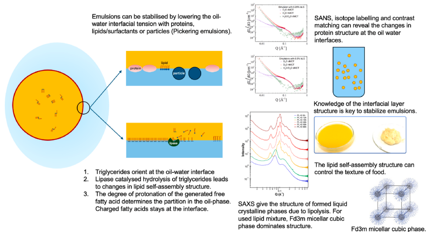
Fig. 3. Schematic illustration of how the interfacial processes can affect the stability of the emulsion and the lipid self-assembly structure. The SANS data is for \beta -lactoglobulin stabilized emulsions of MCT-oil at pH 7. The data for is for two protein concentrations 0.25 % (top) and 0.5 % (bottom). To separate out the contributions for the different components different isotopic contrasts are used, D 2 O and d-MCT-oil highlights the protein, D 2 O and h-MCT-oil highlights the oil, H 2 O/D 2 O (60/40 ratio) and d-MCT-oil matches out the protein, while H 2 O and h-MCT-oil matches out bulk oil but give weak protein contrast. Data from Heiden-Hecht et al. (Heiden-Hecht et al., 2024). The SAXS data from Gladkauskas et al. show the effect of adding lipase to oat oil samples that contains 40 wt% polar lipids (Gladkauskas et al., 2025). The photo to the right shows the texture of the sample after different incubation time, where the photo to the far right one for the micellar cubic phase (photo kindly provided by Dr. Cecilia Tullberg, Lund University).
