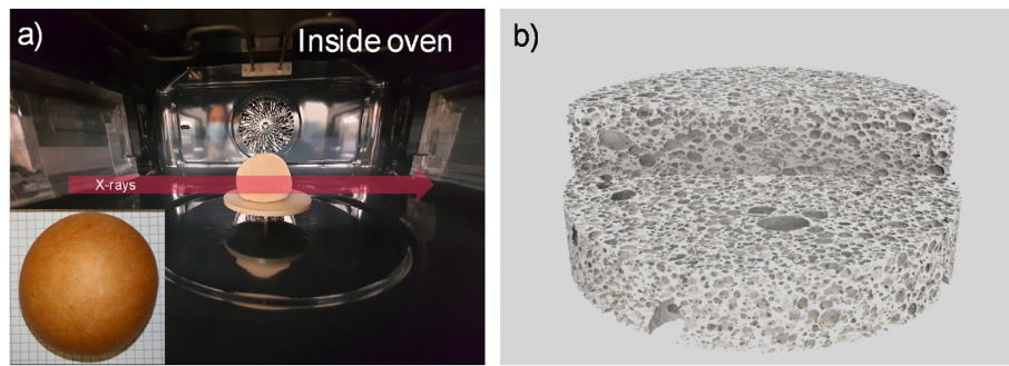
Fig. 4. X-ray tomography imaging of in situ baking inside a combined conventional and microwave oven. a) Image showing the custom-built rotation table inside the oven and a picture of a baked bun. b) 3D structure of the bread close to the beginning of the baking (Schott, Isaksson, et al., 2023).
