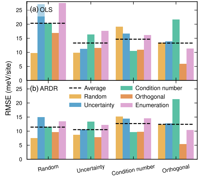
FIG. 6. Comparison of structure generation schemes for the \text{Mo}_{1-x}\text{V}_x\text{C}_{1-y}\square_y system. Here CEs were constructed with the use of four different training sets (as indicated on the x axis) consisting of 110 structures and trained with either (a) OLS or (b) ARDR. The RMSEs were evaluated with use of the different training sets as test sets (as indicated by the bar color), including a set of enumerated structures. The dashed line indicates the average over the five test sets.
