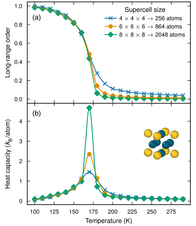
FIG. 11. Order-disorder transition in \text{AuPd}_3 from MC simulations. (a) Long-range order parameter and (b) heat capacity as a function of temperature and system size, where the solid lines are guides for the eye. The system size is given in multiples of the primitive (four-atom) unit cell. The long-range order is represented by the partial static structure factor between Pd atoms. The inset shows the ordered low-temperature phase.
