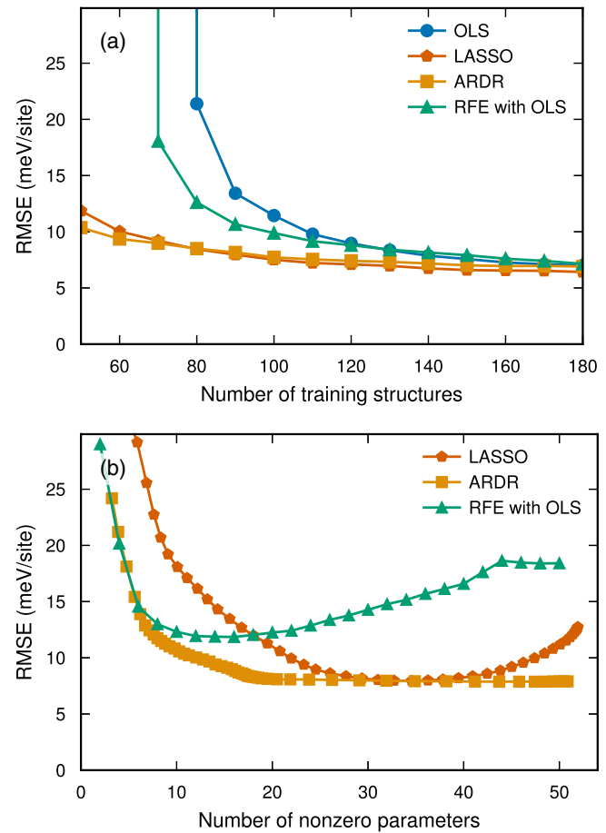
FIG. 2. RMSE obtained with different regression methods in the \text{Mo}_{1-x}\text{V}_x\text{C}_{1-y}\square_y system. (a) Validation RMSE based on the random training set obtained with different regression methods as a function of the number of structures included in the training set. (b) Validation RMSE when 80 training structures are used as a function of the number of nonzero parameters obtained after regression and feature selection. Here the number of nonzero parameters obtained is controlled by variation of the hyperparameter controlling the sparsity of the solution continuously. For ARDR, this is the \lambda -threshold parameter, for LASSO it is \alpha [see Eq. (4)], and for RFE it is the number of features.
