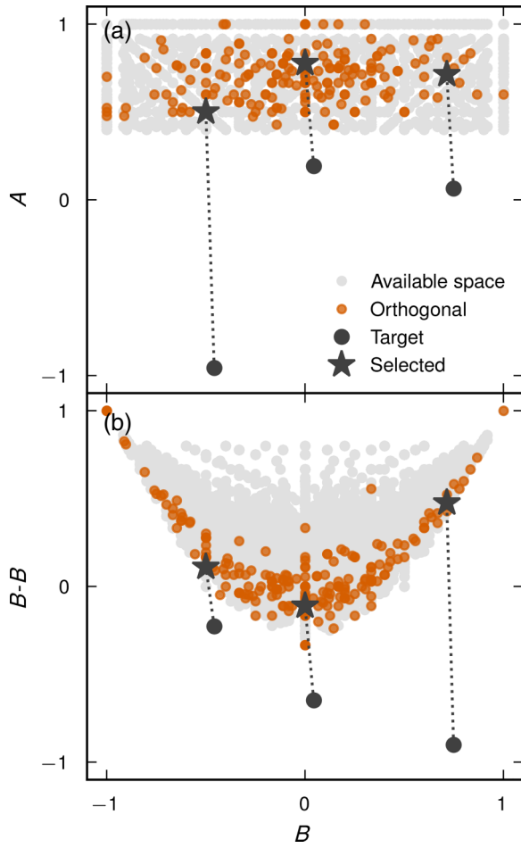
FIG. 5. Correlations between orbits. Correlations between (a) the singlets of the carbon ( A ) and metal ( B ) sublattices and (b) the metal singlet and nearest neighbor. The light-gray area indicates the available space represented by all the structures from the large random pool used for condition number minimization. The orthogonal dataset is shown in orange. The orthogonalization procedure is visualized by the initial (circle) and final (star) positions of three example structures.
