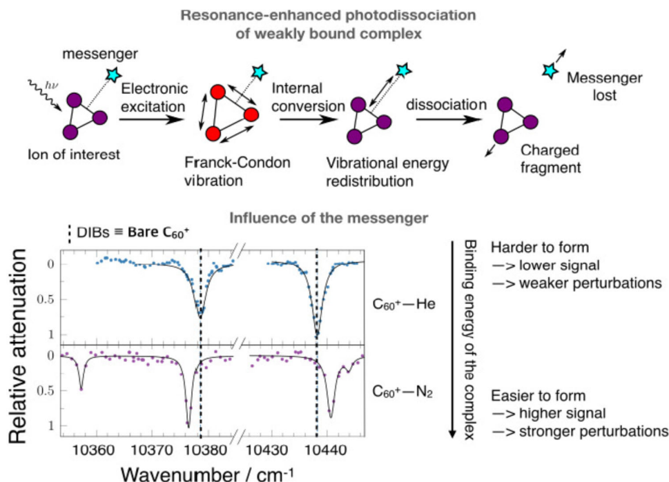
Fig. 6 Messenger spectroscopy of molecular ions. The bottom left is adapted from Ref. [59]
