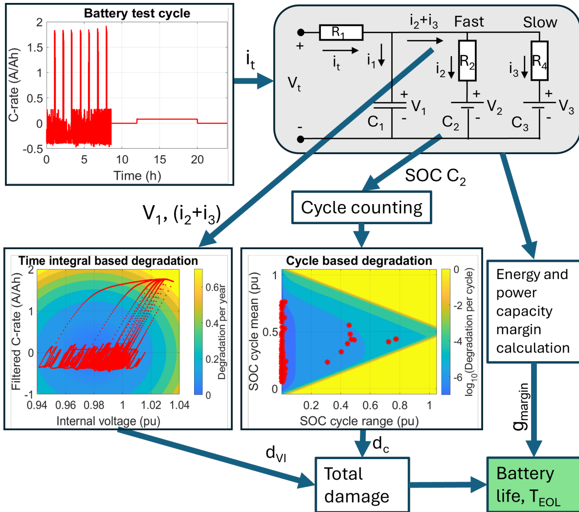
Figure 1: The battery model for cost estimation. The red lines/points which are shown in the diagrams are for the “Fast ch. 5 min every 75 km” case.
