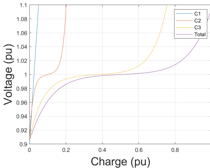
Figure 2: The relation between voltage and charge used for the different parts of the model
