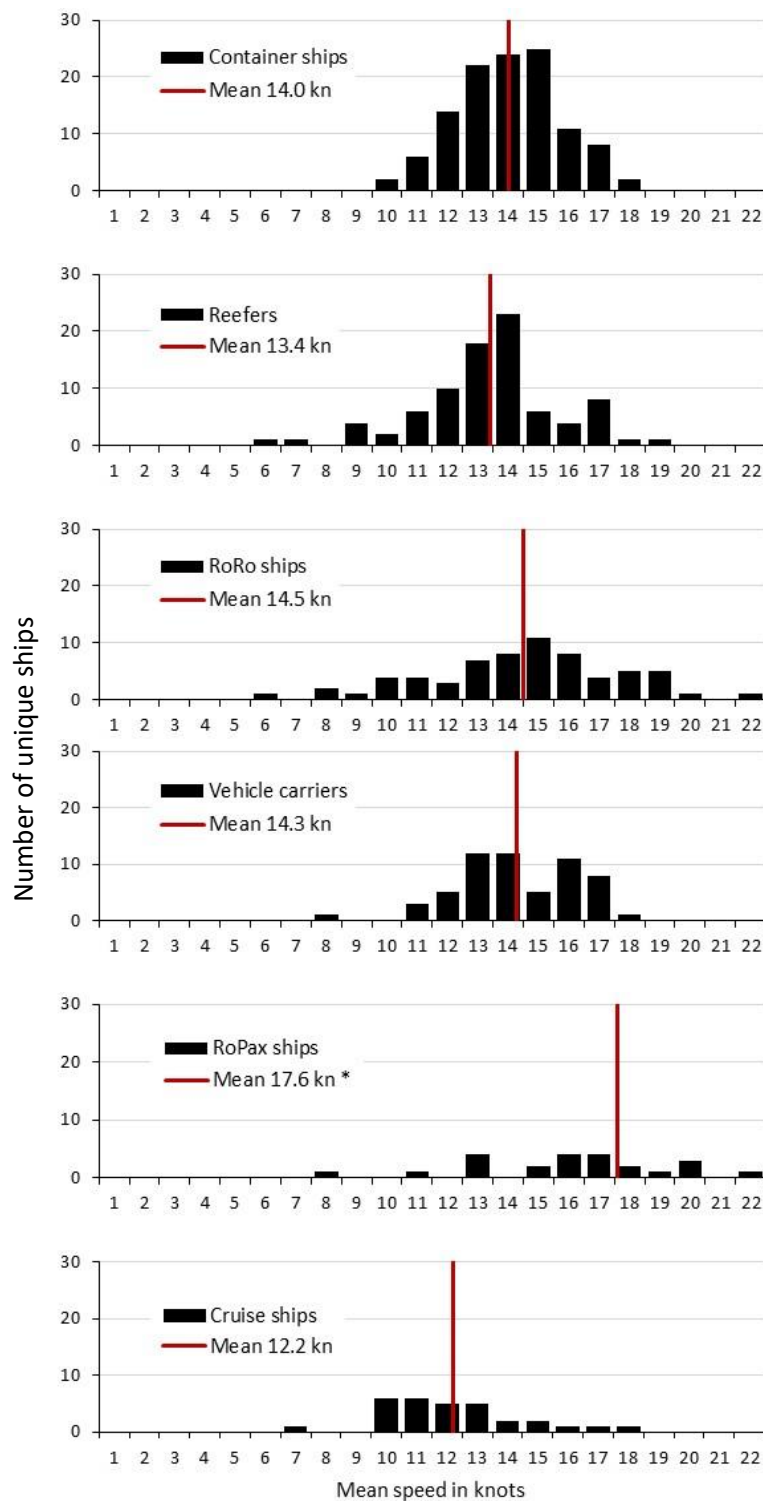
Figure 10. Mean speeds of Container Ships, Reefers, RoRo Ships, Vehicle Carriers, RoPax Ships, and Cruise Ships in the study area in 2021. *The mean speed of three high speed crafts (RoPax Ships) exceeded 22 knots, but these data are not shown in the figure. Note that the scale at the y-axis differs in Figure 10 and Figure 11.
