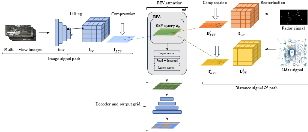
Fig. 1: SMAB architecture. The imaging signal is merged with distance signals from radar and/or lidar to a common voxel grid representation using learnable BEV query and BFA attention mechanism.
