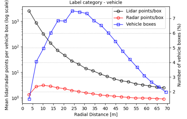
Fig. 4: Comparison of radar and lidar point density in vehicle box versus radial distance w.r.t. the ego-vehicle in the nuScenes [22] dataset. The black and red, circle marked curves represent the mean number of lidar and radar points respectively, for a given distance while the blue, square marked curve indicates the number of boxes of vehicle.
