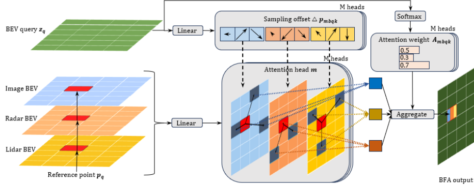
Fig. 2: BFA (BEV feature aggregator) architecture. Compressed multimodal BEV signals are sampled using learned reference point offsets \Delta p_{mbqk} and aggregated for every attention head with learned attention weights A_{mbqk} . See Section III-C for detailed explanation.
