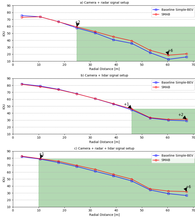
Fig. 3: IOU across radial distances for different sensor setups. The blue square-marked line represents the baseline, while the red circle-marked line represents SMAB. Arrows indicate IOU gains over the baseline, with the green area highlighting improvements. BFA enhances representation, especially when radar/lidar density is low.
