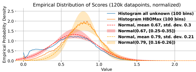
Figure 7: Empirical maximum scores over unknown traffic.
