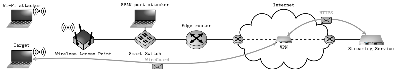
Figure 4: Illustration of the attack and testing environment; note that the testing setup has been designed to facilitate our evaluation and most elements are not required for the attack to be performed.
