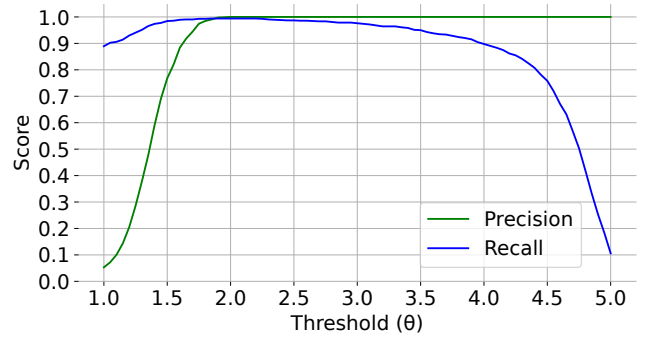
Figure 8: Effect of \theta for 140 hours of known VPN traffic and 490 hours of unknown traffic.
