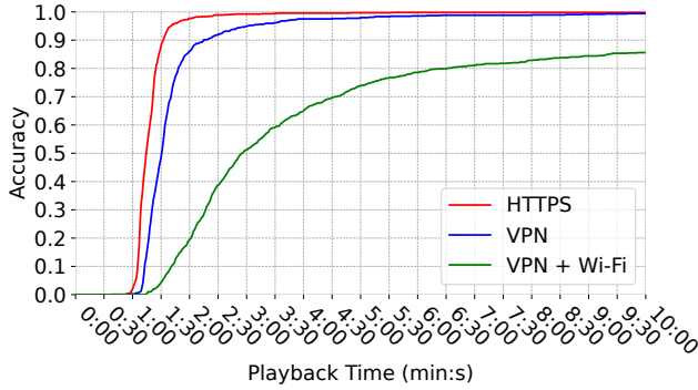
Figure 6: Cumulative accuracy for the evaluated attack scenarios over the playback time.
