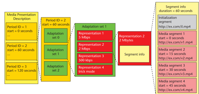
Figure 1: The hierarchical structure of a DASH manifest; source: Sodagar, 2011 [26].
