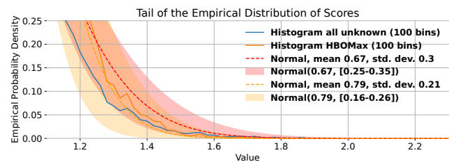
Figure 10: Empirical maximum scores over unknown traffic, tail of the empirical distributions.
