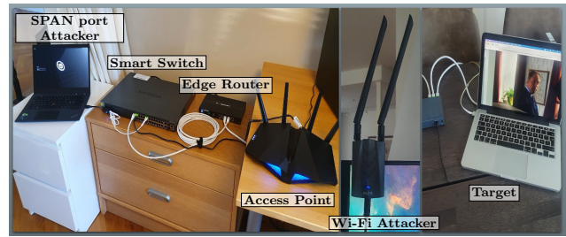
Figure 9: Deployed experimental setting.
