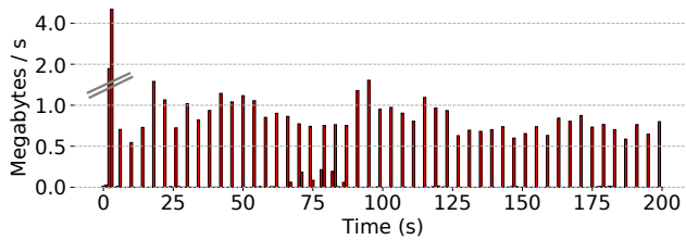
Figure 2: The bursty behavior of ABR streaming, starting off with the buffer-fill before transitioning to the steady state.
