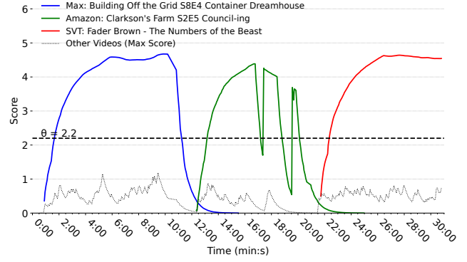
Figure 5: System scoring over time as target streams three videos with a VPN, demonstrating how it adapts over time.
