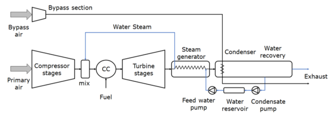
FIGURE 1. Schematic of the SWITCH WET (Water Enhanced Turbofan) engine including the steam generator (vaporizer) component located aft of the gas turbine core (steam turbine not shown) (Reproduced from Stefanizzi et al [11])
