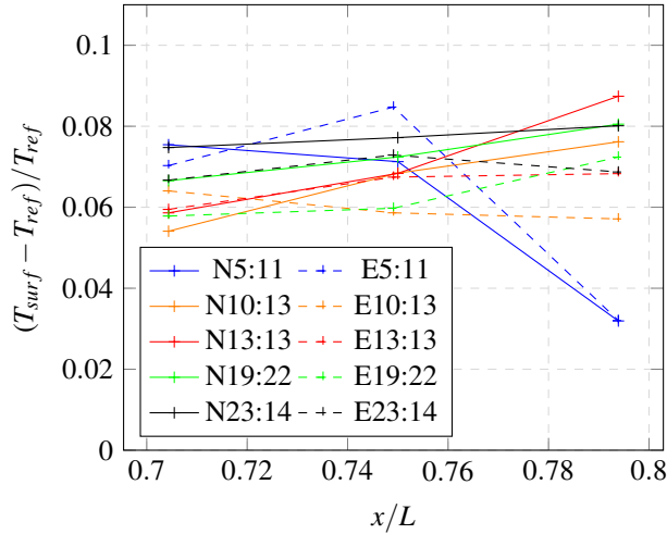
FIGURE 13. Temperature increase relative to the inlet temperature T_{ref} (vertical axis) vs. normalized axial position (horizontal axis) when heated with constant input power Q in segment 8. "N" and "E" denote numerical and experimental results, respectively, with locations as per Fig. 4; e.g., numerical values at row 5, column 11 are labeled N5:11.
