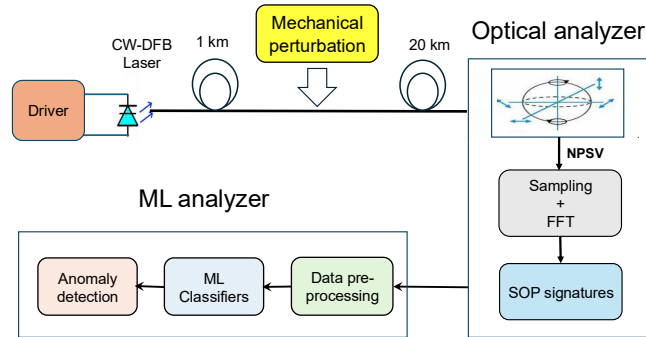
Figure 1: Schematic of the experimental testbed used for polarization signature analysis. Mechanical disturbances are applied between the 1 km coupling fiber and the 20 km fiber spool.
