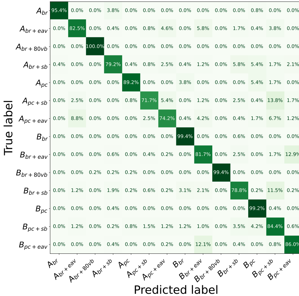
Figure 2: Results of Confusion Matrix for Histogram Gradient Boosting classifier
